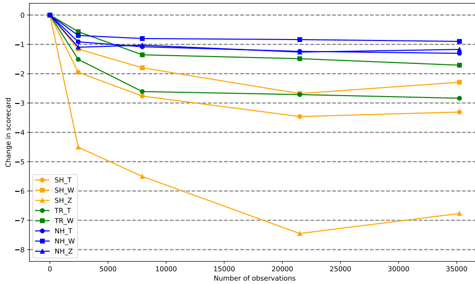
Figure 22. Change in the RMSE scorecard Average percentage reduction in RMSE across scorecard variables and lead times as a function of the number of observations for variables in different latitude regions. Only variables at 850, 500 and 250 hPa have been included in the calculation. Verification against sonde observations. The number of observations shown is an approximate figure calculated before quality control. Note that the 20,000 occultations per day experiment shown here is the default one provided by EUMETSAT.
