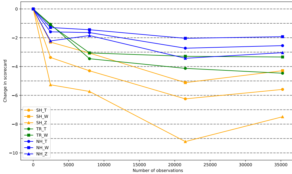
Figure 25. Change in the RMSE scorecard for the different variables Average percentage reduction in RMSE across scorecard lead times and variables at 850, 500 and 250 hPa as a function of the number of observations for variables in different latitude regions. Verification against ECMWF analyses. The number of observations shown is an approximate figure calculated before quality control. Note that the 20,000 occultations per day experiment shown here is the default one provided by EUMETSAT.
