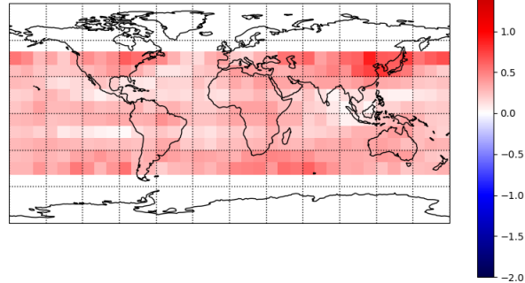
Figure 16. Mean difference between the observations and the model background of the observations, normalised by their average. Calculated within a system which does not account for tangent-point drift using COSMIC-2 observations. The data are averaged over all the ROMEX observations, but binned by latitude and longitude.
