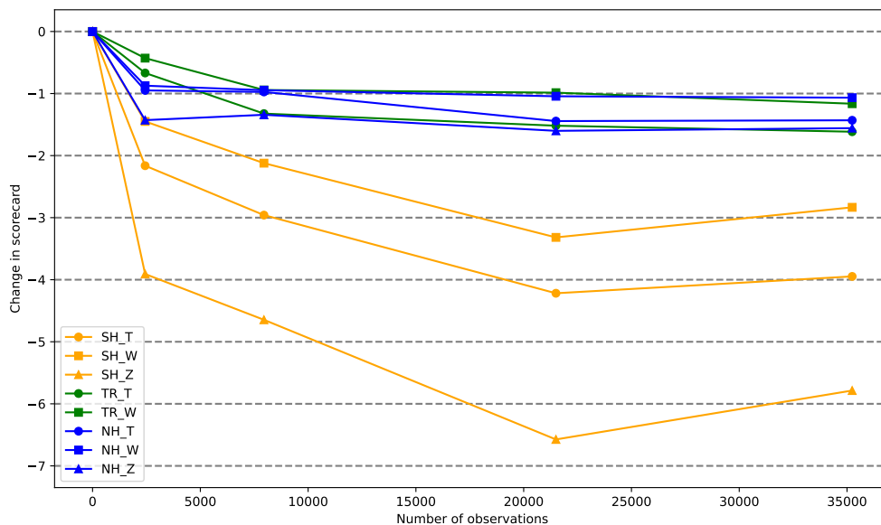
Figure 24. Change in the RMSE scorecard for the different variables Average percentage reduction in RMSE across scorecard lead times and variables at 850, 500 and 250 hPa as a function of the number of observations for variables in different latitude regions. Verification against sonde observations. The number of observations shown is an approximate figure calculated before quality control. Note that the 20,000 occultations per day experiment shown here is the default one provided by EUMETSAT.
