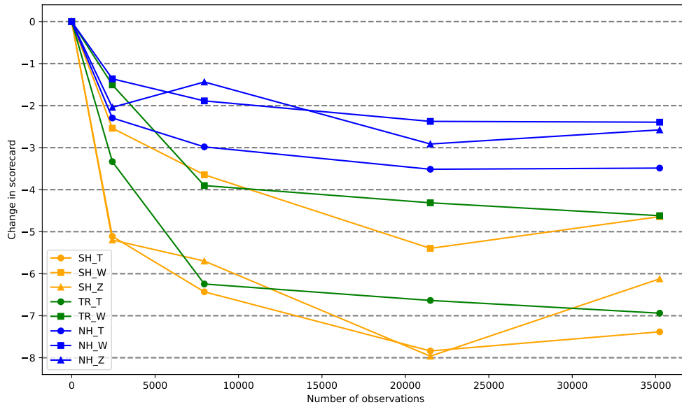
Figure 23. Change in the RMSE scorecard Average percentage reduction in RMSE across scorecard variables and lead times as a function of the number of observations for variables in different latitude regions. Only variables at 850, 500 and 250 hPa have been included in the calculation. Verification against ECMWF analyses. The number of observations shown is an approximate figure calculated before quality control. Note that the 20,000 occultations per day experiment shown here is the default one provided by EUMETSAT.
