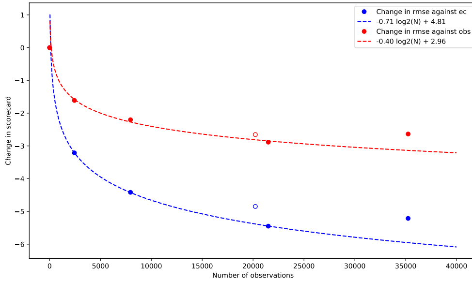
Figure 19. Change in the overall RMSE scorecard. Average percentage reduction in RMSE across scorecard variables and lead times for the different experiments. Verification against ECMWF analyses is shown in blue, and verification against observations is shown in red. A best-fit curve based on a variation of the overall figure with the logarithm of the number of observations is shown as the dashed line. The curve has been fit to the experiments using Control - COSMIC-2, control, and 20,000 occultations per day. The number of observations shown is an approximate figure calculated before quality control. The hollow circle indicates the results from the alternative 20,000 occultations per day experiment.
