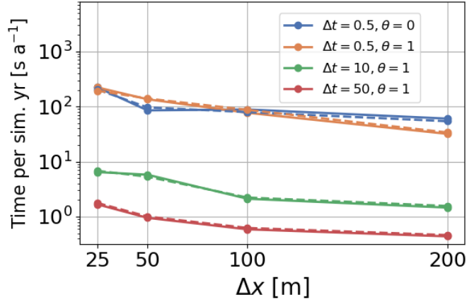
Figure 7. The average CPU time (solid lines) and the wall time (dashed lines) per simulation year for MISIMIP Exp. 3a over 500 simulation years starting at t = 10000 year. The colours indicate the time step size, \Delta t , and whether the FSSA is active ( \theta = 1 ) or inactive ( \theta = 0 ). Results are shown for refined horizontal mesh resolutions of 25, 50, 100, and 200 m.
