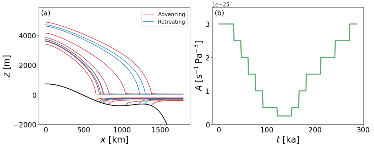
Figure 3. The MISIMIP Exp. 3a (Pattyn et al., 2012) is designed to demonstrate grounding line migration over prograde and retrograde slopes, see the solid black line showing the bed elevation in (a). The movement of the grounding line is induced by altering the ice fluidity, A , at certain intervals during transient simulation as seen in (b). As the ice fluidity is reduced, the grounding line advances (red lines, (a)) and as the ice fluidity is increased, the grounding line retreats (blue lines, (a)).
