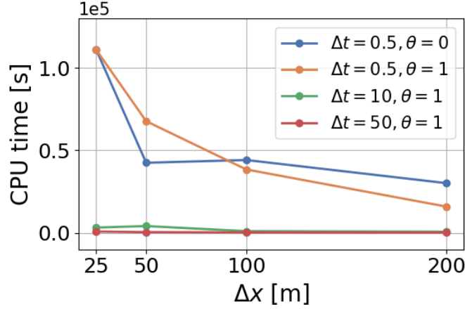
Figure 7. The CPU time for MISMIP Exp. 3a for 500 simulation years starting at t = 10000 year. The colours indicate the time step size, \Delta t , and whether the FSSA is active ( \theta = 1 ) or inactive ( \theta = 0 ). Results are shown for refined horizontal mesh resolutions of 25, 50, 100, and 200 m.
