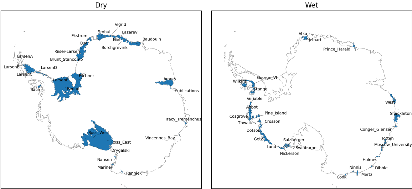
Figure B1. Maps of Antarctic ice shelves classified into dry (left) and wet (right) climates, separated by the median snowfall threshold of 500 \text{ mm yr}^{-1} . Labels indicate the ice shelves within each category.
