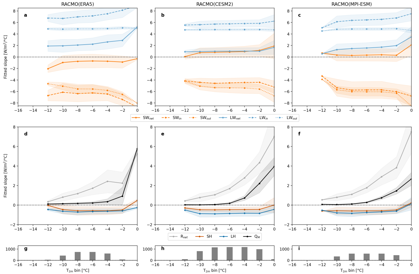
Figure 9. As in Fig. 8 but for ice shelves in wet climates (annual precipitation > \sim 500 mm)
