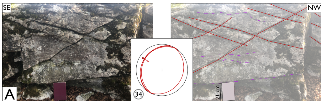
Figure 7. Field example from the Salève. A conjugate pair of reverse shear fractures at low angle with the bedding define the reverse association SA1. For legend see figure 3E.
