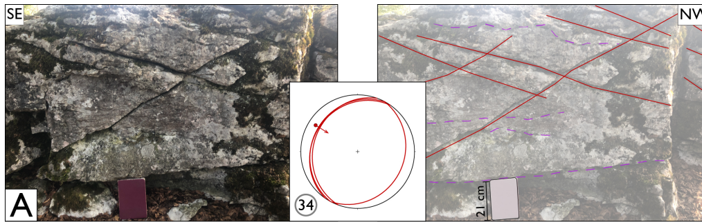
Figure 7. Field example from the Salève. A conjugate pair of reverse shear fractures small-scale faults at low angle with the bedding define the reverse association SA1. For legend see figure 3E.
