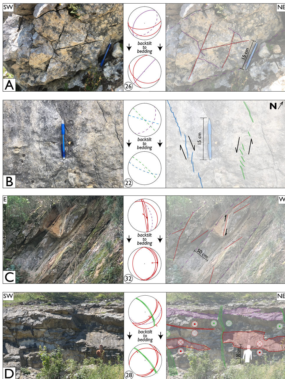
Figure 6. Field examples from the Jura. A Reverse shear fractures-small fault with low angle with respect to the bedding, in association with a bed-perpendicular stylolite together form the reverse association JA1. B Top view of a bedding surface displaying a conjugate pair of vein arrays. Together with similarly oriented bed-perpendicular shear fractures-faults they form a strike-slip association JA2. C Tilted shear fractures-small-scale faults at low angle with respect to the bedding. The strike after backtilting is \sim N-S. They form the reverse association JA3. D Reverse fractures of JA1 are cross-cut by bed-perpendicular, sinistral shear fractures-faults of JA4. The plunge of the slickensides on these the shear fractures-planes indicates they formed prior to tilting of the bedding. For legend see figure 3E.
