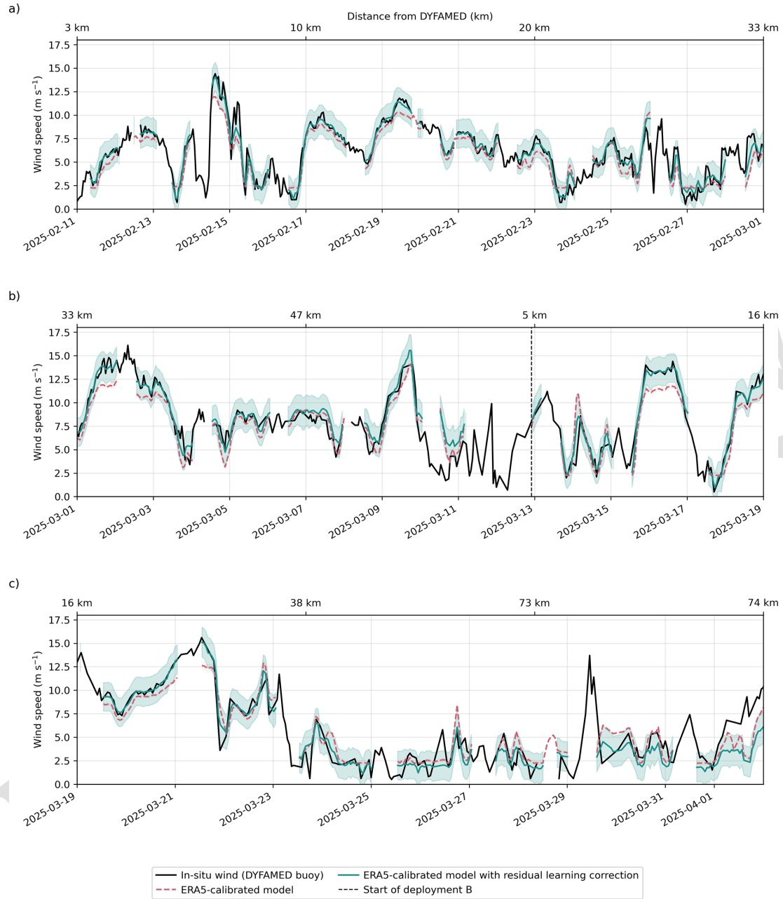
Figure 8. Time series comparison between acoustic float wind estimates and DYFAMED buoy winds, displayed over three consecutive 18 d windows (a–c). The dashed pink curve corresponds to wind speeds predicted using the Nystuen et al. (2015) acoustic model calibrated solely with ERA5 reanalysis winds. The solid blue line shows the same model after applying the residual-learning correction (XGBoost), and the shaded region indicates its associated predictive uncertainty. Buoy-measured wind speed is shown in black. The upper x -axis reports the float's distance from DYFAMED throughout the record, and the dashed vertical line indicates the transition to deployment B.
