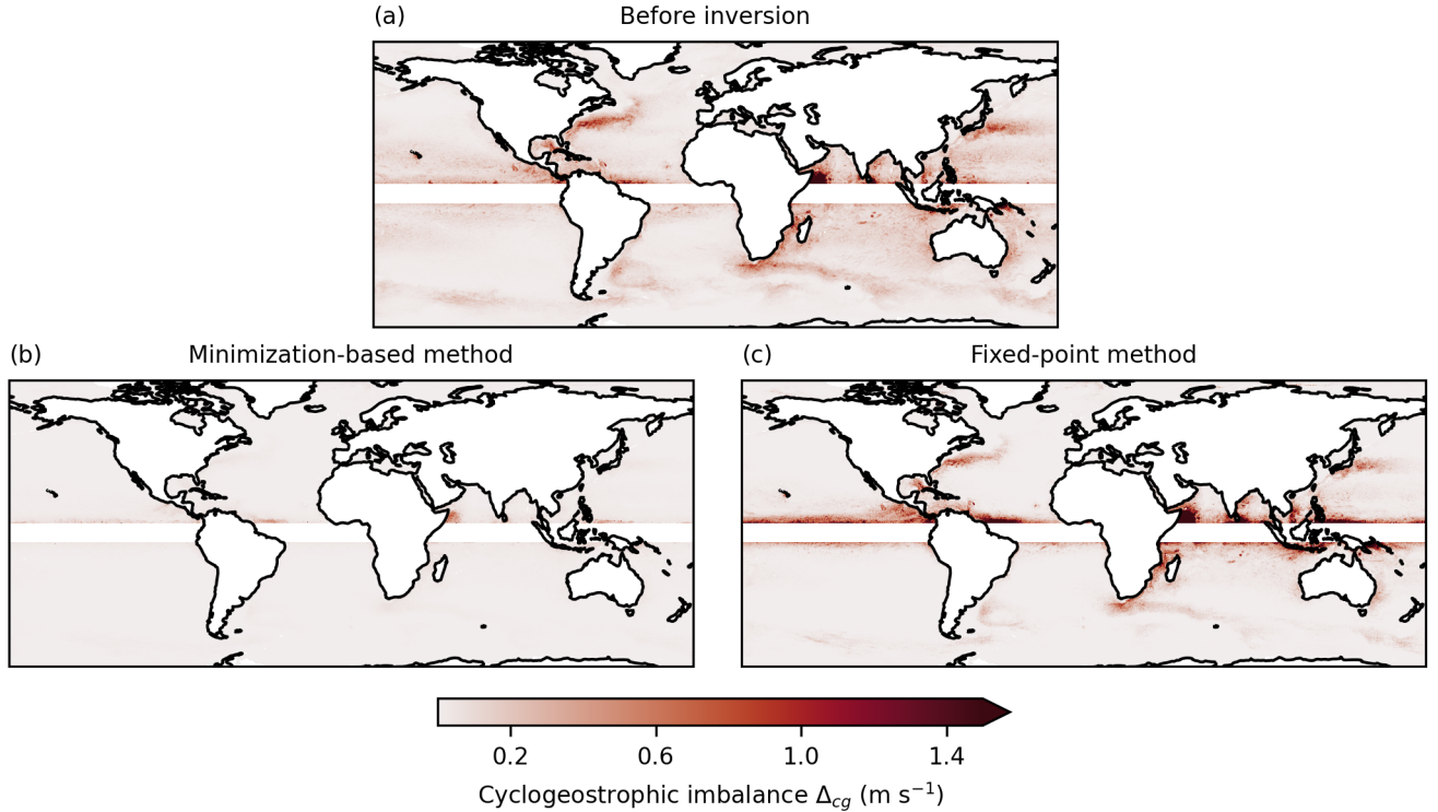
Figure 1. Maps of cyclogeostrophic imbalance, computed from Eq. 9, for the geostrophic velocity (a), the minimization-based cyclogeostrophic velocity (b), and the fixed-point cyclogeostrophic velocity (c) derived from NeurOST SSH.
