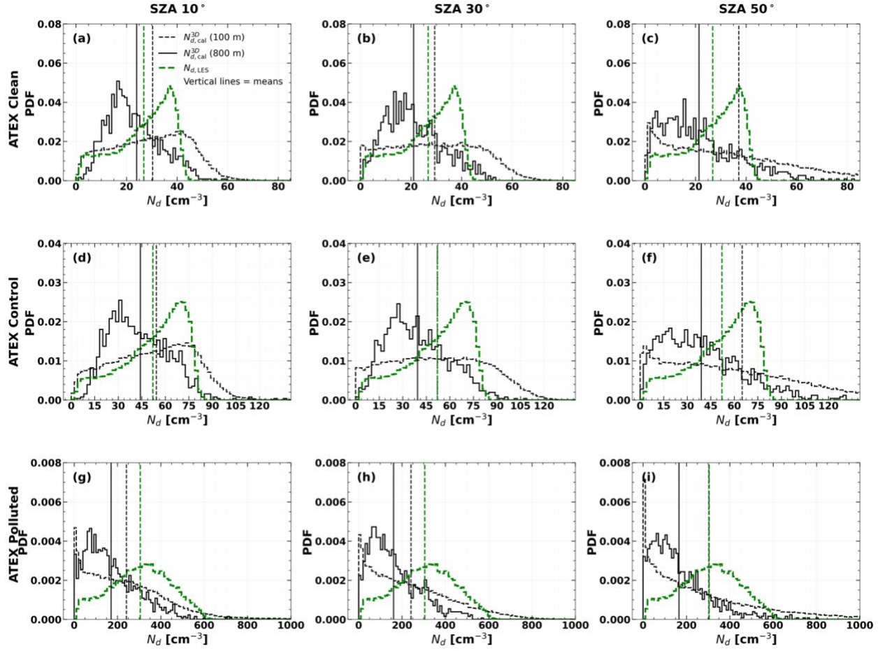
Figure 6. Probability Density Functions (PDFs) comparison of N_{d,cal}^{3D}(2.1\mu m) for LES (100 m) and coarse satellite-like (800 m) resolution for all cloudy pixels, at SZA 10^\circ , 30^\circ and 50^\circ for the ATEX clean, control and polluted case across all time steps. Vertical lines represent mean values. The green line represents the LES reference ( N_{d,LES} )
