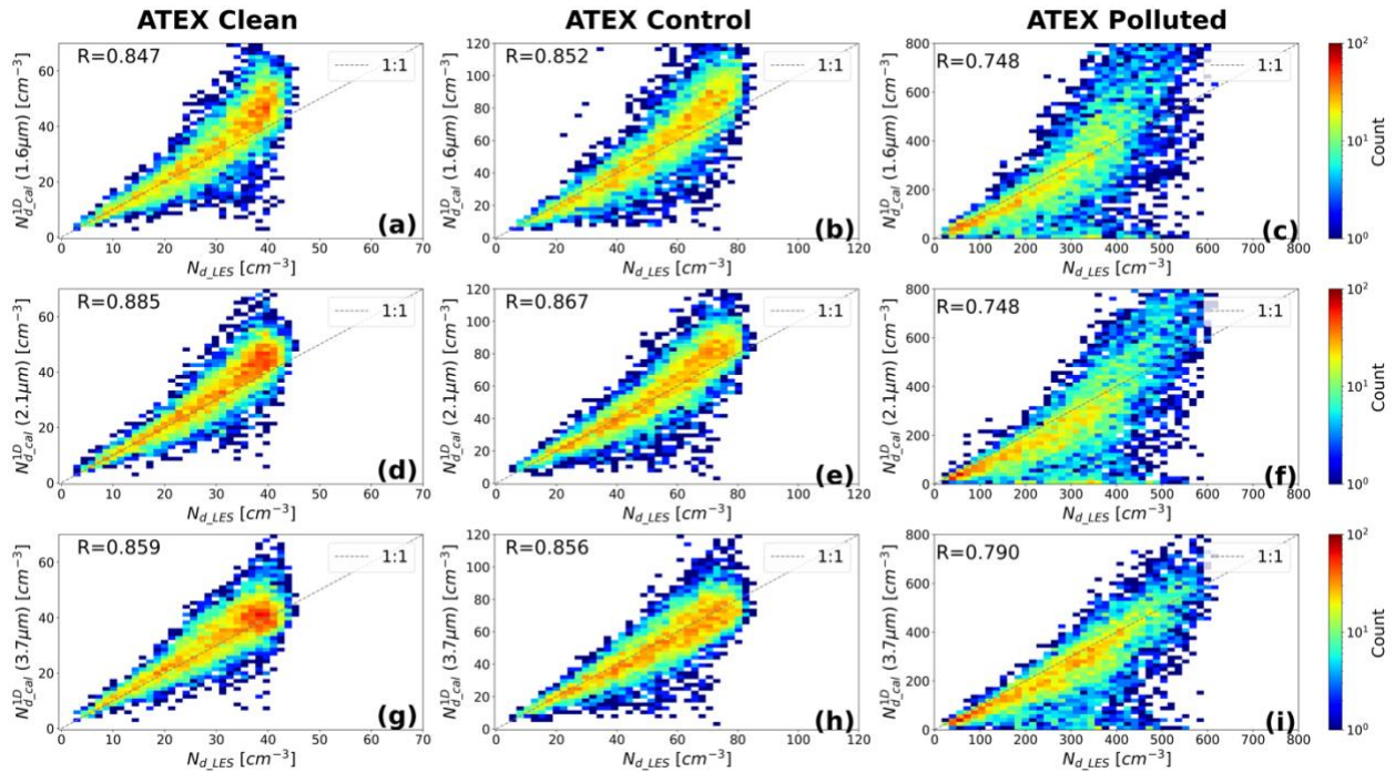
389 Figure 2. Comparison of N_d derived from bi-spectral retrievals based on 1D RT reflectance ( N_{d\_cal}^{1D}(\lambda_{abs}) ) versus 390 N_d obtained from the LES ( N_{d\_LES} ) for (a) ATEX clean, (b) ATEX control and (c) ATEX polluted for retrievals at 391 absorbing channel, ( \lambda_{abs} ) of 1.6 \mu m , for (d) ATEX clean, (e) ATEX control and (f) ATEX polluted for retrievals at 392 \lambda_{abs} of 2.1 \mu m and for (g) ATEX clean, (h) ATEX control and (i) ATEX polluted for retrievals at \lambda_{abs} of 3.7 \mu m 393 at 4 h of simulation time. Note: 1D RT and bi-spectral retrievals utilized for this comparison were carried out at SZA 394 50^\circ . Dotted lines indicate 1:1 relationship between the derived and LES N_d .
