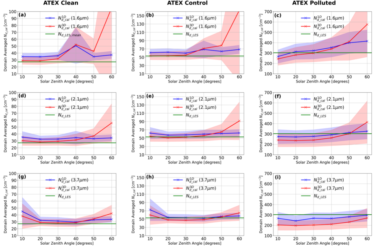
Figure 5. Domain average of N_{d\_cal}^{1D}(\lambda_{abs}) and N_{d\_cal}^{3D}(\lambda_{abs}) as a function of solar zenith angle as well as domain average of the N_{d\_LES} reference for the ATEX clean, ATEX controlled and ATEX polluted case averaged across all time steps for \lambda_{abs} = 1.6, 2.1 , and 3.7 \mu m . The shaded region is the associated standard error computed from the population variance. Note that the y scale is different for each LES case due to the range of N_d associated with each LES case.
