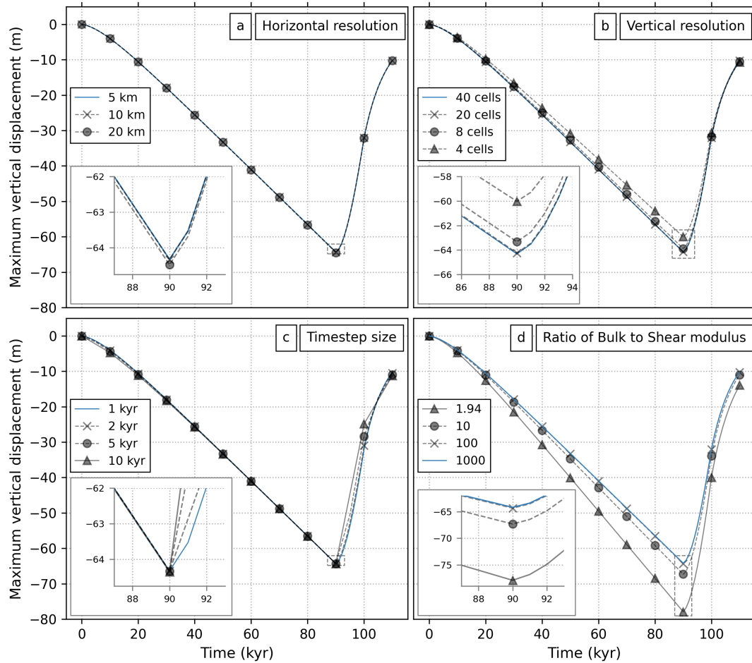
Figure 4. Sensitivity analysis for G-ADOPT using the scenario explored in Figure 3b consisting of long-duration ice loading on a 1D Earth model. (a) Impact of horizontal resolution. Solid blue = default spacing (5 km beneath ice sheet, 200 km in far field); crosses = half of default resolution; circles = one quarter of default resolution. (b) Impact of vertical resolution. Solid blue = default case with 40 vertical cells across the model domain (i.e., 10 per layer); crosses = 20 cells; circles = eight cells; triangles = four cells. (c) Impact of timestep size. Solid blue = default of 1 kyr; crosses = 2 kyr; circles = 5 kyr; triangles = 10 kyr. (d) Impact of transitioning from incompressible to a realistic Earth-like level of compressibility by modifying the ratio of bulk-to-shear modulus. Solid blue = 1000; crosses = 100; circles = 10; triangles = 1.94.
