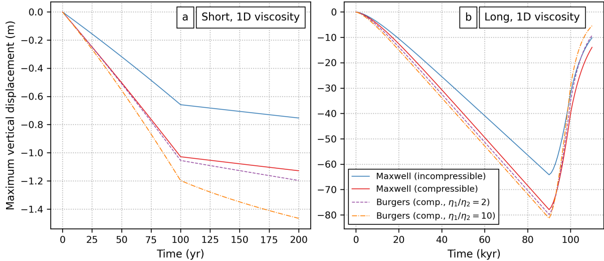
Figure 5. Extension of the 3D Cartesian benchmark to a compressible Burgers rheology. (a) Short-duration loading scenario on a 1D Earth model. Solid blue = incompressible Maxwell rheology previously shown in Figure 3a; solid red = equivalent for compressible Maxwell rheology (bulk-to-shear modulus ratio of 1.94) shown in Figure 4d; dashed purple = Burgers rheology with short-term viscosity a factor of 2 lower than the long-term viscosity; dash-dotted orange = same for a factor of 10 viscosity reduction. (b) Same for the long-duration loading scenario.
