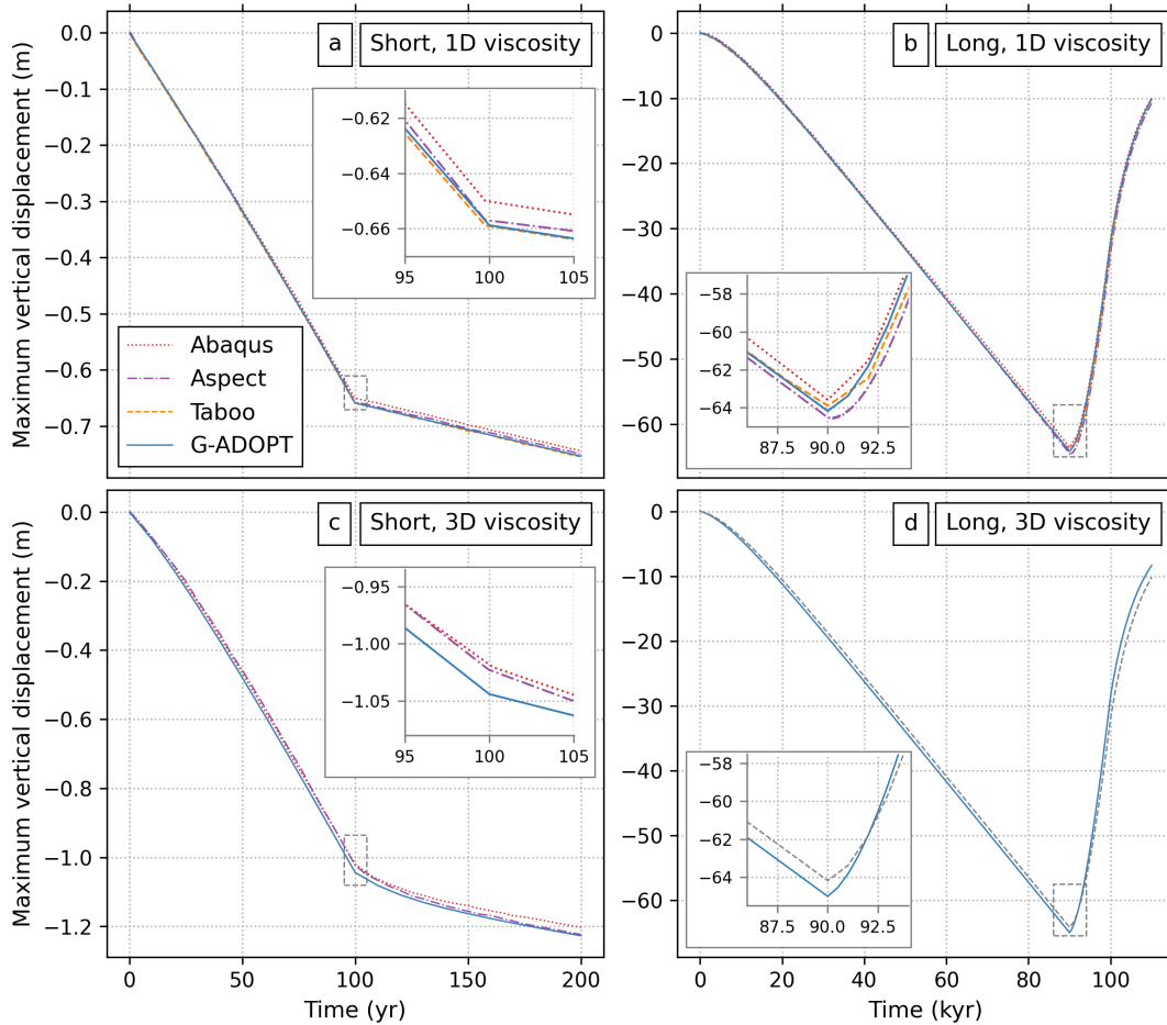
Figure 3. Comparison of maximum vertical surface displacements beneath the ice load for the 3D Cartesian box benchmark scenarios of Weerdesteijn et al. (2023) . (a) Short-duration loading scenario on a 1D Earth model. Dotted red = Abaqus; dash-dotted purple = Aspect; dashed orange = Taboo; and solid blue = G-ADOPT. Inset shows a zoom of the region outlined by the black-dashed box. (b) Same for the long-duration loading scenario on a 1D Earth. (c) Short-duration loading scenario on a 3D Earth containing a low-viscosity patch in the upper mantle beneath the ice sheet. (d) Same for the long-duration loading scenario on a 3D Earth; grey dashed line = G-ADOPT result on a 1D Earth (panel b) plotted to highlight impact of the low-viscosity patch. Note that results for Abaqus, Aspect and Taboo are digitised from Weerdesteijn et al. (2023) and that not all some of the four scenarios illustrated were not tested in those codes. Also note the different displacement extent on each y-axis extends for the short- versus long-duration scenarios .
