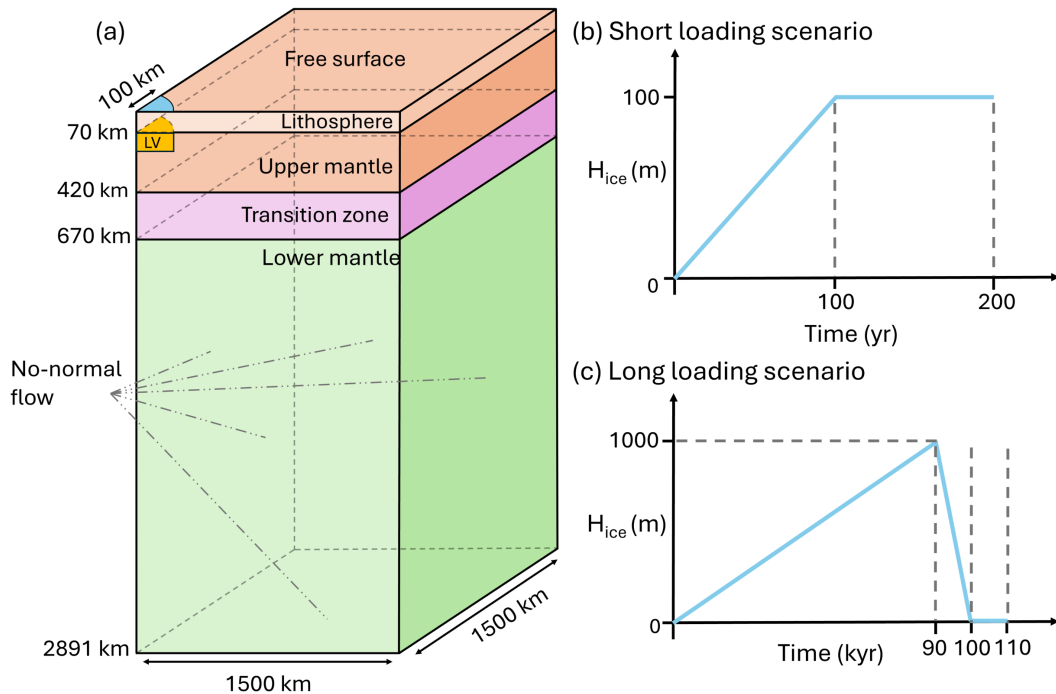
Figure 2. Schematic of the 3D Cartesian benchmark from Weerdesteijn et al. (2023) . (a) Model domain showing rheological layers, an optional low viscosity (LV) zone, and the extent of ice at the surface. Note schematic is not drawn to scale. (b) Temporal evolution of thickness of the ice disk in the short-loading scenario. (c) Same for the long-loading scenario.
