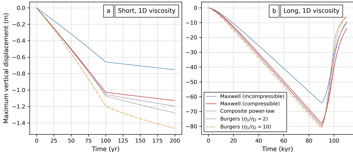
Figure 5. Extension of the 3D Cartesian benchmark to a-compressible Burgers rheology non-Maxwell rheologies . (a) Short-duration loading scenario on a 1D Earth model. Solid blue = incompressible Maxwell rheology previously shown in Figure 3a; solid red = equivalent for compressible Maxwell rheology (bulk-to-shear modulus ratio of 1.94) previously shown in Figure 4d; dotted black = composite power-law rheology with transition stress \tau_T = 0.2 MPa and exponent n = 3 ; dashed purple = Burgers rheology with short-term viscosity a factor of 2 lower than the long-term viscosity; dash-dotted orange = same for a factor of 10 viscosity reduction. (b) Same for the long-duration loading scenario.
