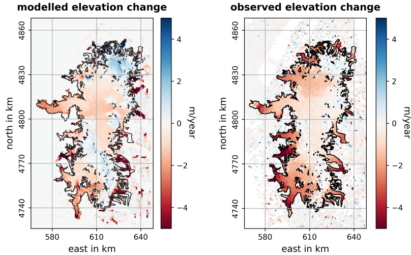
Figure 5. Modelled (left) and observed (right) elevation changes for 2000-2014.
