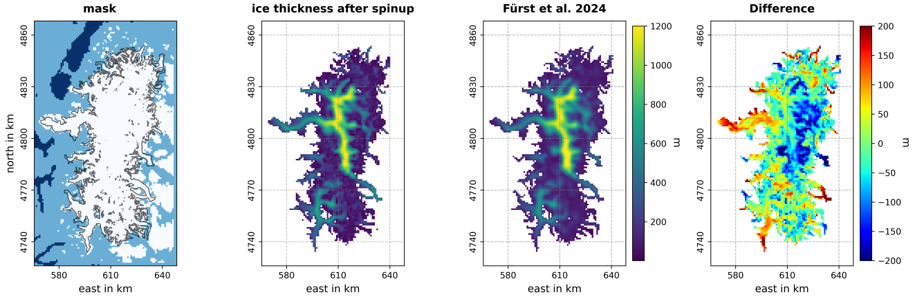
Figure 3. Comparison of the NPI state after the spin-up to observations; left: modelled mask (white: ice, light blue: land, dark blue: ocean) and observed year 2000 outlines (black contour), middle: modelled ice thickness after the spin-up clipped to the year 2000 outlines for a better comparison, right: modelled ice thickness for the year 2000 by Fürst et al. (2024).
