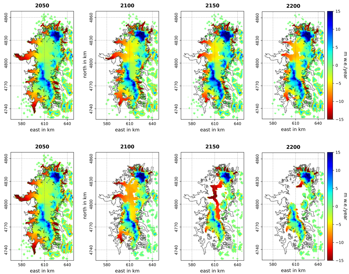
Figure A2. Surface mass balance of the projected ice bodies in the NPI area.
