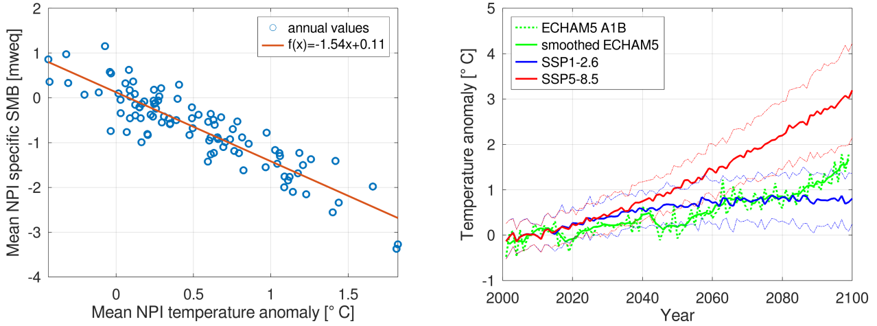
Figure 2. Left: Relationship of NPI averaged surface mass balance and temperature anomalies for the 21st century (from Schaefer et al. (2013)). Right: Temperature anomalies over the NPI as projected by the ECHAM5-Model (A1B scenario, green lines) (Roeckner et al., 2003) and the mean (red and blue solid lines) \pm one standard deviation (discontinuous lines) of 33 CMIP6 models (Table A2). The selected reference period for the anomalies is 2000–2015.
