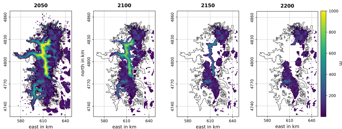
Figure 8. Simulated ice thickness of the NPI in the 21st and 22nd centuries under the SSP5-8.5 scenario. Year 2000 icefield outlines are shown for comparison.
