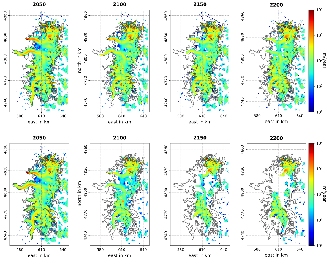
Figure A3. Ice speed of the projected ice bodies of the NPI area.
