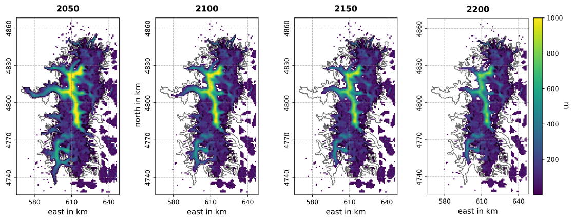
Figure 7. Simulated ice thickness of the NPI in the 21st and 22nd centuries under the SSP1-2.6 scenario. Year 2000 icefield outlines are shown for comparison.
