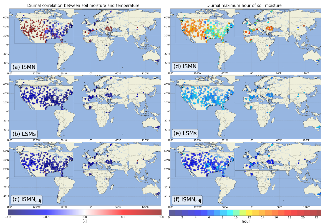
Figure 6: Spatial distribution of the temporal correlation coefficient of hourly time series of surface soil moisture (SM) and temperature (TS) from (a) ISMN, (b) the mean of land reanalysis datasets (LSMs: ERA5-Land and MERRA-2), and (c) ISMN adj , where red triangles and blue circles indicate positive and negative correlation coefficient, respectively. The diurnal maximum phase of surface SM in (d) ISMN, (e) LSMs, and (f) ISMN adj .
