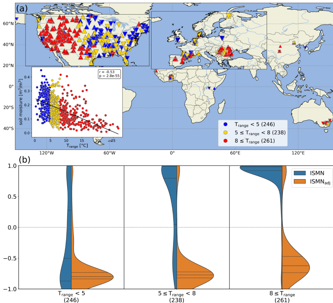
Figure 7: (a) Spatial distribution of correlation coefficients between diurnal cycles of SM and TS from ISMN, classified by T_{range} , where upward- and downward-pointing triangles indicate positive and negative correlations, respectively. The lower-left scatter plot shows the relationship between climatological DTR and SM, where colors correspond to the same DTR range used in the map. The spatial correlation coefficient along with its corresponding p-value is also shown. (b) Violin plots of the probability distribution of correlation coefficients (on Y axis) of ISMN (blue) and ISMN adj (orange), in the same three categories according to T_{range} . The bracketed numbers below the x-axis represent the number of stations classified in each DTR category. The total number of stations is decreased to 745, compared with Fig. 1, because only sites with concurrent SM and TS records for at least 92 days are used to calculate the correlation coefficient between variables.
