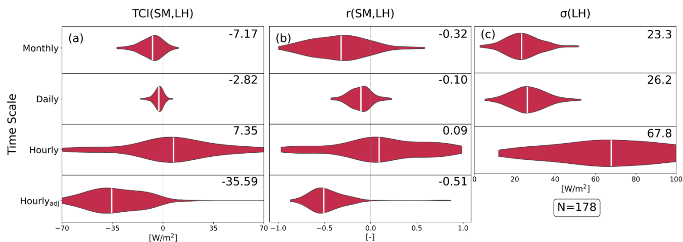
Figure 9: Violin plot of land coupling and its components from flux tower observations (N=178) in monthly (top row), daily (second row), and hourly (third row) and diurnally adjusted hourly (bottom row) timescale during the hemispheric warm season (Northern and Southern Hemisphere MJJAS and NDJFM, respectively). Since the diurnal adjustment is conducted only on the SM time series, the standard deviation term remains identical to the diurnally unadjusted result. (a) TCI(SM, LH) is used to measure the strength of the land coupling, which is a term multiplied by (b) the correlation coefficient between SM and LH and (c) the standard deviation of LH. The values in the upper-right corner of each panel indicate the median value.
