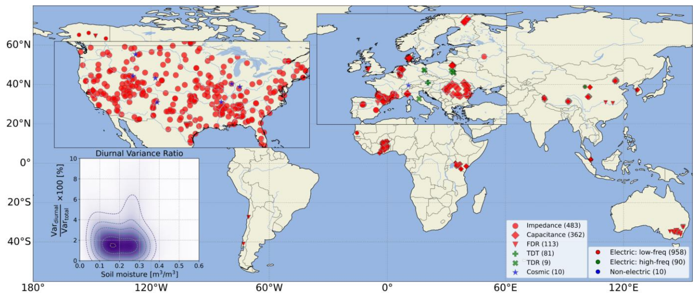
590 Figure 1: Locations of in-situ observation sites of SM (N=1058) from the International SM Network (ISMN). Red and blue dots indicate sensors that use electrical properties (dielectric constant) to observe SM and do not use that method, respectively. Sensors that operate at high frequencies, insensitive to temperature biases, are shaded green. The lower-left figure shows the ratio of diurnal variance against total variance in the SM measurements. The bracketed numbers in the lower-right legend denote the number of sites adopting each corresponding sensor.
