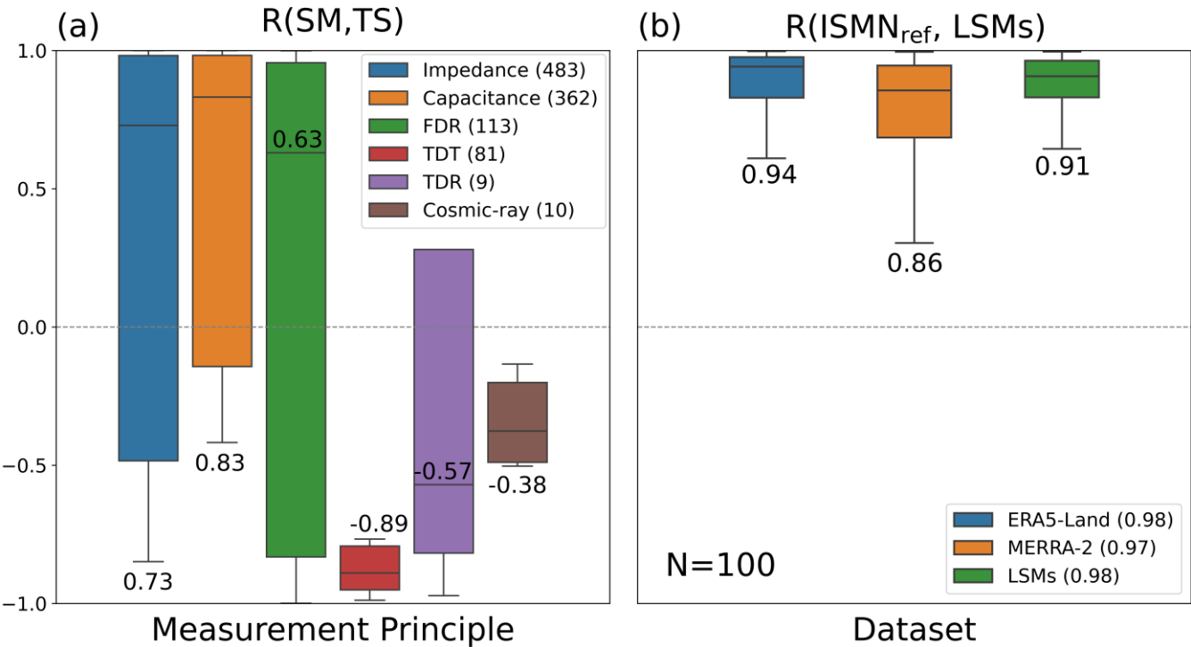
595 Figure 2: Boxplot of the temporal correlation within the diurnal cycle of (a) hourly time series of surface SM and soil temperature for each sensor used to measure SM and (b) modelled surface SM against reference sensors (those with a negative correlation to 600 diurnal temperature: TDT, TDR, and cosmic-ray), where median values are denoted beside each boxplot. Values in parentheses in the legend represent (a) the number of stations using each sensor type for measuring SM, and (b) the correlation between the 24- hour diurnal cycles of reference and modelled SM, based on 24-hour cycles constructed by median values across 100 stations at each hour. LSMs (green) indicate the averaged SM time series from ERA5-Land (blue) and MERRA-2 (orange).
