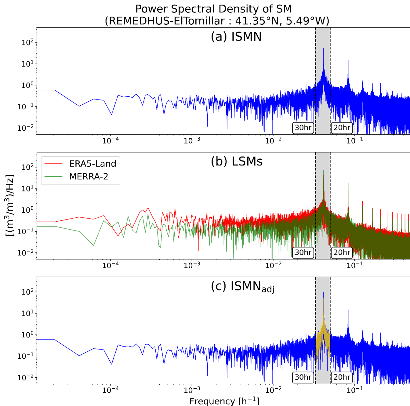
Figure 4: Power Spectral Density (PSD) analysis of surface SM from (a) in-situ measurement, (b) reanalysis datasets (red: ERA5-Land, and green: MERRA-2), and (c) diurnally adjusted in-situ measurement at REMEDHUS-EITomillar station (41.35°N, 5.49°W). The gray shaded area in each panel represents the adjusted frequency windows and the black dotted vertical lines indicate the 20- and 30-hour variance domains. The yellow line in (c) represents the original power of surface SM in the diurnal time window.
