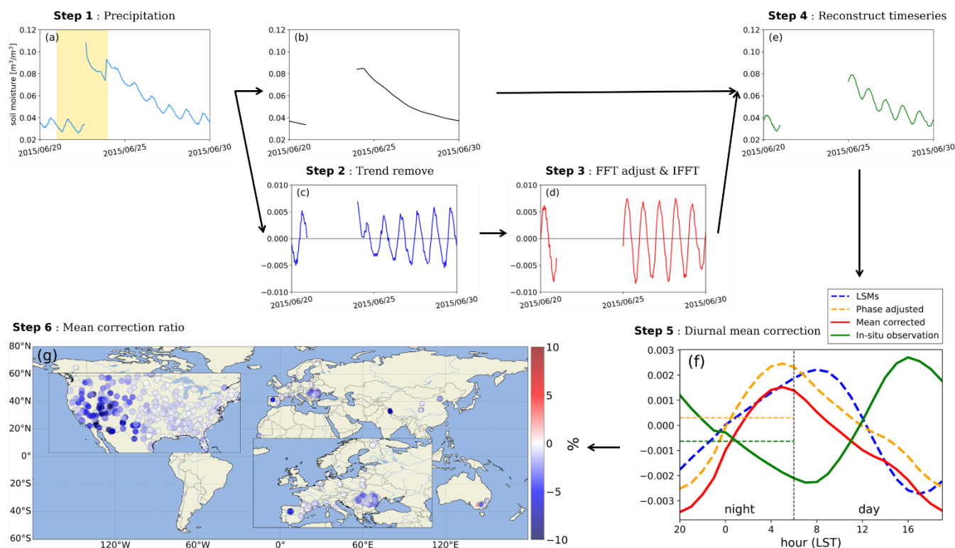
Figure 3: Data preprocessing steps for example station REMEDHUS- ElTomillar (41.35°N, 5.49°W): (a) Removal of days with precipitation events, with yellow shading indicating precipitation dates. (b) Running mean calculated using a 24-hour centered moving average. (c) SM anomaly derived by subtracting (b). (d) Adjusted SM anomaly using the Fourier Transform method. (e) Reconstruction of time series obtained by adding (d) and (b). (f) Diurnal time series showing the original in-situ observation (green), model-based data (blue dashed line), phase adjusted data (yellow dashed line), and the final adjusted result (red line). (g) Mean corrected ratio over the global map, with negative percentages in blue and positive percentages in red.
