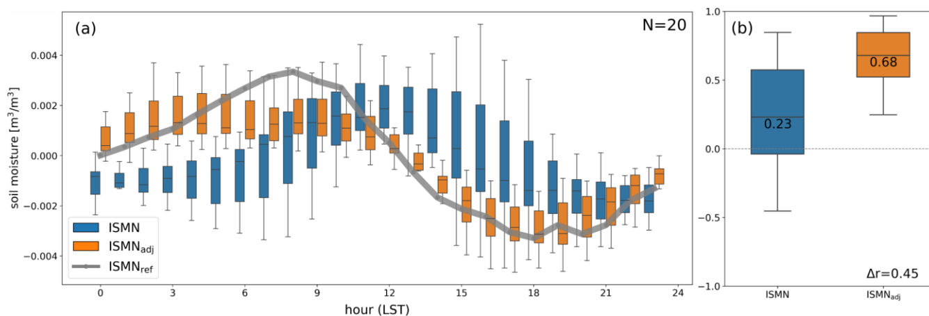
620 Figure 5: (a) Diurnal cycle of surface SM, filtered by a 24-hour running mean from electrical-based ISMN (blue), ISMN adj (orange boxplot), and reference sensors (gray line). To compare the impact of diurnal adjustment on electric-based measurements with the reference sensors, the 20 closest electric-based observations are sampled within 200 km from the reference sensors. (b) Boxplot of the temporal correlation coefficient of diurnal time series of surface SM from electrical-based ISMN (blue) and ISMN adj (orange) against the corresponding reference observations.
