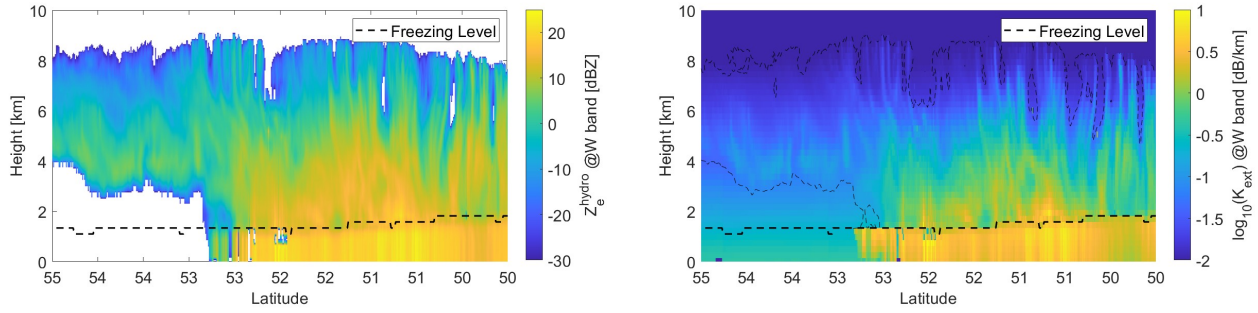
Figure 6. W-band vertical profiles of effective reflectivity (left) and W-band hydrometeor extinction coefficient (right) in correspondence to the microphysical properties shown in Fig. 5. The dashed black line corresponds to the freezing level.
