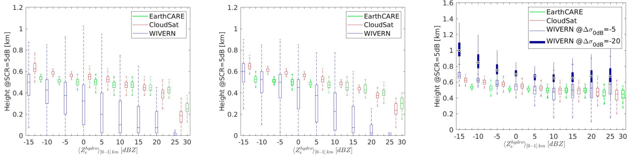
Figure 13. Box plots of the distributions of H_{SCR=5\text{ dB}} as a function of the mean value of \langle Z_e^{hydro} \rangle_{[0-1]\text{ km}} for oceanic rainfall (left), snowfall (center) and snowfall over land or sea-ice (right). In the box plots the central mark indicates the median and the bottom and top edges of the box indicate the 25th and 75th percentiles, respectively whereas the whiskers extend to the most extreme data points not considered outliers. In the right panel, there are two box plots for WIVERN corresponding to a \Delta\sigma_0 = -5\text{ dB} and 20\text{ dB} , respectively.
