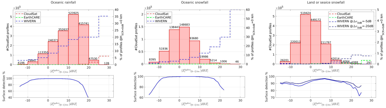
Figure 14. Top: Number of CloudSat profiles selected for statistical analysis, for oceanic rainfall on the left, oceanic snowfall in the middle panel, and land or sea ice snowfall on the right; profiles are clustered by effective reflectivity in surface classes from -15dBZ to 30dBZ, each 5dBZ wide. Dashed lines are the percentage of profiles detected at ground level ( H_{@SCR=5dB} = 0km ) and are shown for WIVERN (blue), CloudSat (red) and EarthCARE (magenta). Bottom: Proportion of profiles detected by WIVERN compared to those detected by CloudSat as a function of \langle Z_e^{hydro} \rangle_{[0-1] km} . The profiles detected by Cloudsat are the 100% baseline. Results are only shown for reflectivity classes with more than 100 profiles.
