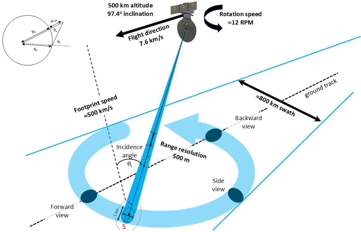
Figure 1. WIVERN geometry of observation with the conical scanning pattern with all the nomenclature used in Sect. 2. The width of the footprint is exaggerated for illustration purposes.
