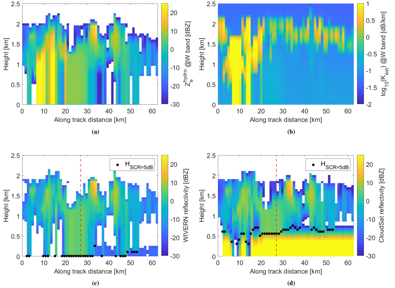
Figure 11. Reconstruction of WIVERN and CloudSat observations for the oceanic snowfall event whose ground track is shown in the right panel of Fig. 4. Top panels: hydrometeor effective reflectivity (a) and extinction coefficient (b) at W band. Bottom panels: WIVERN (c) and CloudSat (d) simulated measured reflectivity.
