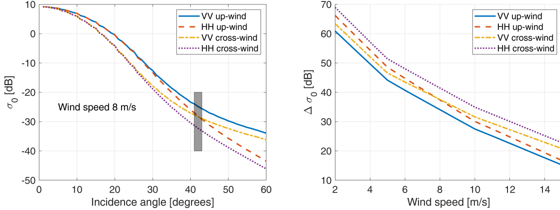
Figure 3. Left panel: \sigma_0 dependence on the incidence angle for an ocean surface with wind speed of 8 m/s for different polarization and for up-wind and cross-wind observations as indicated in the legend. The geophysical model is based on the work by Battaglia et al. (2017). The grey rectangle corresponds to the value expected for WIVERN. Right panel: the reduction in \sigma_0 when moving from nadir to slant observations at 42^\circ .
