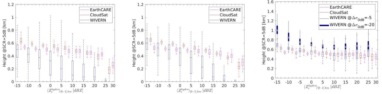
Figure 13. Box plots of the distributions of H_{SCR=5\text{ dB}} as a function of the mean value of \langle Z_e^{\text{hydro}} \rangle_{\text{angle}[0-1]\text{ km}} for oceanic rainfall (left), snowfall (center) and snowfall over land or sea-ice (right). In the box plots the central mark indicates the median and the bottom and top edges of the box indicate the 25th and 75th percentiles, respectively whereas the whiskers extend to the most extreme data points not considered outliers. In the right panel, there are two box plots for WIVERN corresponding to a \Delta\sigma_0 = -5\text{ dB} and -20\text{ dB} , respectively.
