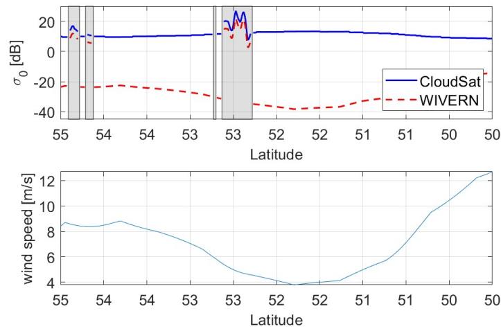
Figure 7. Left-Top panel: simulated \sigma_0 for nadir looking radar like CloudSat (blue line) and for a 42^\circ incidence angles (WIVERN)(red dashed line). Note that over land a \Delta\sigma_0 = 5 dB has been assumed. Right-Bottom panel: wind speed to show the dependence of WIVERN \sigma_0 from it. Shaded areas correspond to land where the \sigma_0 is assumed to be independent of the incidence angle.
