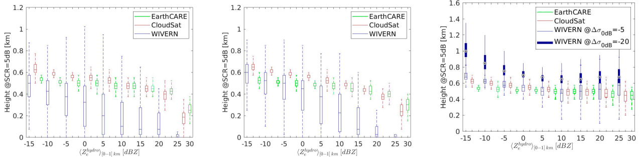
Figure 13. Box plots of the distributions of H_{SCR=5 \text{ dB}} as a function of the mean value of \langle Z_e^{\text{hydro}} \rangle_{[0-1] \text{ km}} for oceanic rainfall (left), snowfall (center) and snowfall over land or sea-ice (right). In the box plots the central mark indicates the median and the bottom and top edges of the box indicate the 25th and 75th percentiles, respectively whereas the whiskers extend to the most extreme data points not considered outliers. In the right panel, there are two box plots for WIVERN corresponding to a \Delta\sigma_0 = -5 \text{ dB} and 20 \text{ dB} , respectively.
