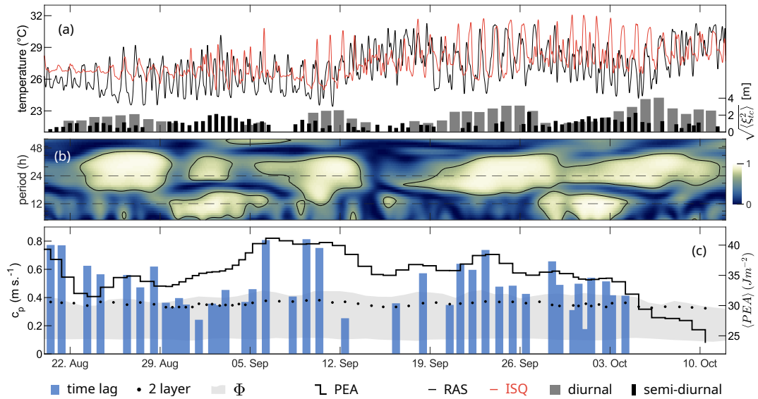
Figure 5. Cross-shelf coherence analysis. (a) Temperature time series at 18 m depth from stations RAS (black) and ISQ (red). Bars represent \xi_{\text{rms}} for the D- (grey) and SD- (black) components, as shown in Fig. 3e. (b) Wavelet coherence between the two temperature series, emphasizing the tidal frequency band (D- and SD-periods are marked by dashed lines). (c) Phase speed based on time lags between RAS and ISQ (blue bars), derived from modal analysis (shaded grey area) and two-layer model (points). Phase-averaged PEA (solid black line) is shown on the right y-axis.
