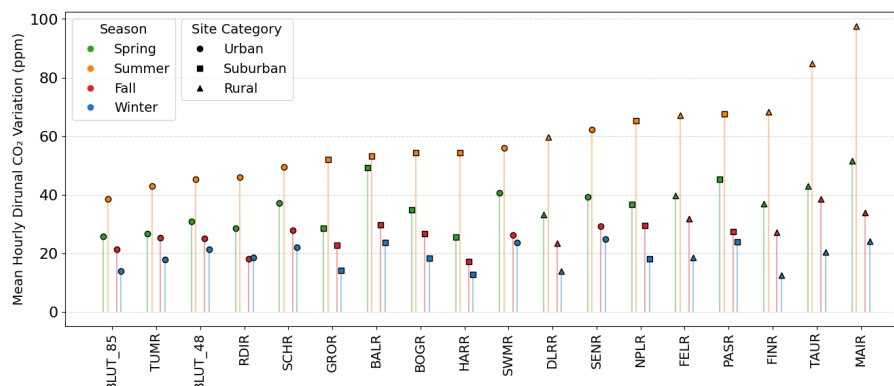
Figure 13. Seasonal diurnal variation in hourly aggregated CO 2 concentrations across all ACROPOLIS sites. The diurnal variation is defined as the daily maximum minus minimum CO 2 concentration. Stations are marked by symbol according to site type: urban, suburban, and rural. The results reveal distinct seasonal and spatial patterns in diurnal CO 2 variability.
