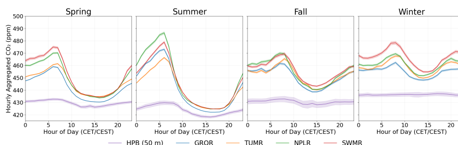
Figure 12. Seasonally averaged diurnal CO 2 profiles for four ACROPOLIS stations with inlets at 30 m above ground level. The selected stations represent different urban contexts within Munich. For comparison, data from the rural ICOS station Hohenpeißenberg (HPB) are also shown. Shaded areas indicate the 95 % confidence interval.
