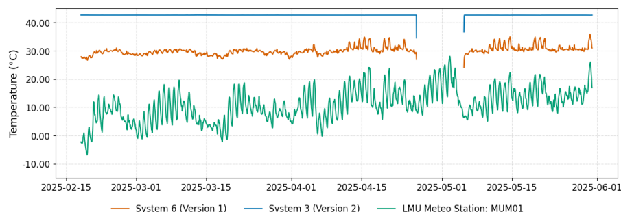
Figure 7. Time series of sensor temperature during field deployment at TUMR (February–June 2025). The plot shows internal GMP343 temperature readings from a first-generation (red) and a second-generation (blue) ACROPOLIS system, alongside outside temperature measured at 30 meters by a nearby meteorological station (green). The generation 2 system exhibits stable temperature control and no apparent response to solar radiation, in contrast to the more variable readings from the generation 1 system. The gap in the time series shows a power outage.
