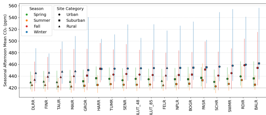
Figure 14. Seasonal afternoon CO 2 concentrations across all ACROPOLIS sites. Measurements are filtered for local afternoon hours (12:00–18:00), then averaged per season. Vertical bars indicate the 2.5 % and 97.5 % quantiles. The plot reveals clear seasonal patterns in CO 2 concentrations and a distinct separation between urban/suburban and rural sites.
