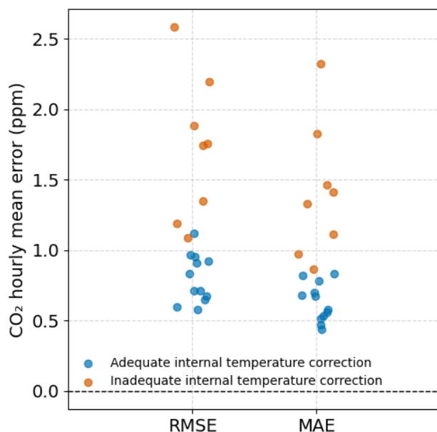
Figure 6. Performance metrics from the 2024 side-by-side comparison of first-generation ACROPOLIS systems. The plot shows root mean square error (RMSE) and mean absolute error (MAE) for each sensor compared to a Picarro G2301 reference instrument. Blue and red colors indicate the effectiveness of internal temperature compensation, with red marking sensors that show inadequate correction and heightened sensitivity to temperature variations.
