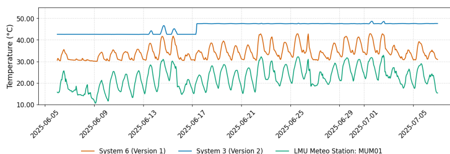
Figure E1. Time series of sensor temperature during field deployment at the TUMR site (June–July 2025). The plot shows internal GMP343 temperature readings from a first-generation (red) and a second-generation (blue) ACROPOLIS system, along with ambient temperature measured at 30 meters above ground by a nearby meteorological station (green). The temperature setpoint for the second-generation system was increased to 45 °C to assess its suitability under elevated summer conditions. The higher target temperature results in a more stable and decoupled sensor environment.
