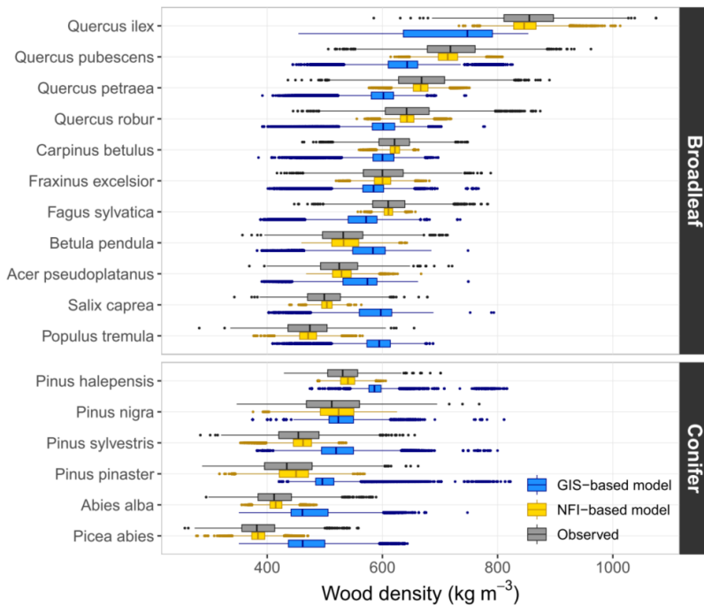
485 Figure 5: Wood density values predicted on the French NFI dataset and values observed in the XyloDensMap data selected for modelling. Observed values correspond to measurements on wood increment cores, while predicted values were obtained from the “NFI-based model” (orange/yellow) and the “GIS-based model” (blue) developed on these measurements. Results are shown for a subset of 17 species.
