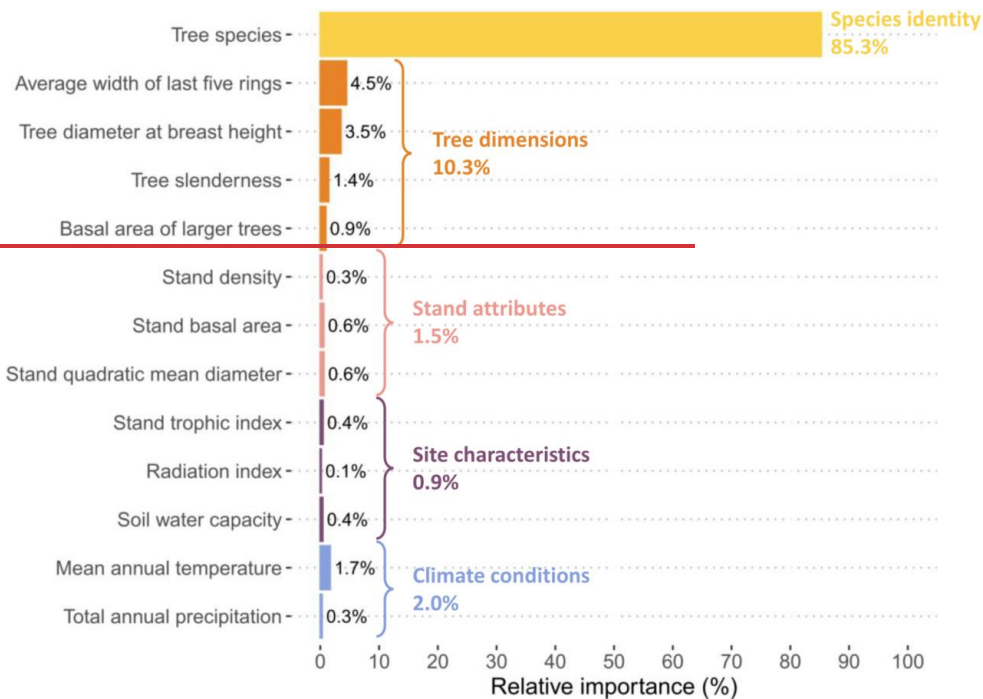
390 Figure 2: Relative importance (in %) of predictive variables in the “NFI-based model” of wood density variation. Variable importance was estimated using the lmg method. For each continuous variable, a species-specific interaction term was included in the model. For average width of the last five rings, tree diameter at breast height, tree slenderness and basal area of larger trees, a log-transformation was applied.
