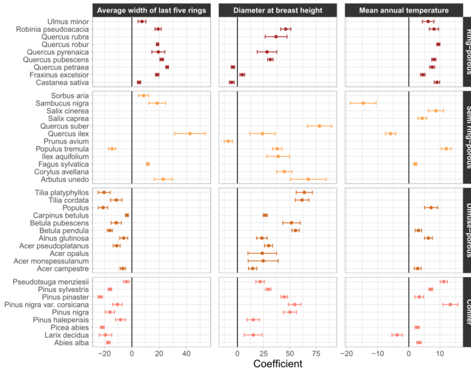
410 Figure 3: Coefficients affected to the average width of the last five tree rings, the diameter at breast height and the mean annual temperature in the “NFI-based model” of wood density variation. Error bars represent the standard error around coefficients. Unsignificant coefficients are not shown. For the average width of the last five tree rings and the diameter at breast height, coefficients are for on the log scale-transformed variable.
