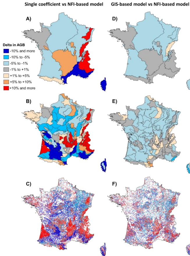
550 Figure 7: Difference in forest aboveground biomass (AGB) stocks depending on the method used to predict wood density: the “NFI- based model”, the “GIS-based model” or a single average coefficient. Comparisons are presented across three spatial levels: biogeographical regions (A and D), biogeographical subregions (B and E), and forest plots inventoried by the French NFI (C and F). Maps on the left show the difference in AGB between estimates derived from the “NFI-based model” and those using the average 555 coefficient. Maps on the right display the difference between estimates derived from the “GIS-based model” and “NFI-based model”. All differences are expressed relative to the AGB estimated using the “NFI-based model”.
