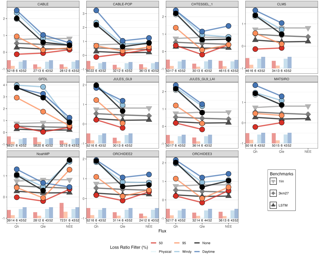
Figure 5. LSM Performance after Application of Different Timestep Filters. The three fluxes are on the x-axis, and the y-axis is the independent normalised metric value iNMV. Note that the y-axis varies for each facet. Each facet is for an individual LSM. Lower iNMV is better. The grey lines are the benchmark EFM, the black line is the original LSM, and the blue and red lines are the LSM under different filters including the 95% and 50% Loss Ratio Filters as well as Daytime, Windy, and Physical filters. The bar charts and labels indicate the percentage of timesteps removed by each of the five filters. Note the differing y-axis scales and that the "Physical" filter is often obscured by the "None" LRF/original model performance.
