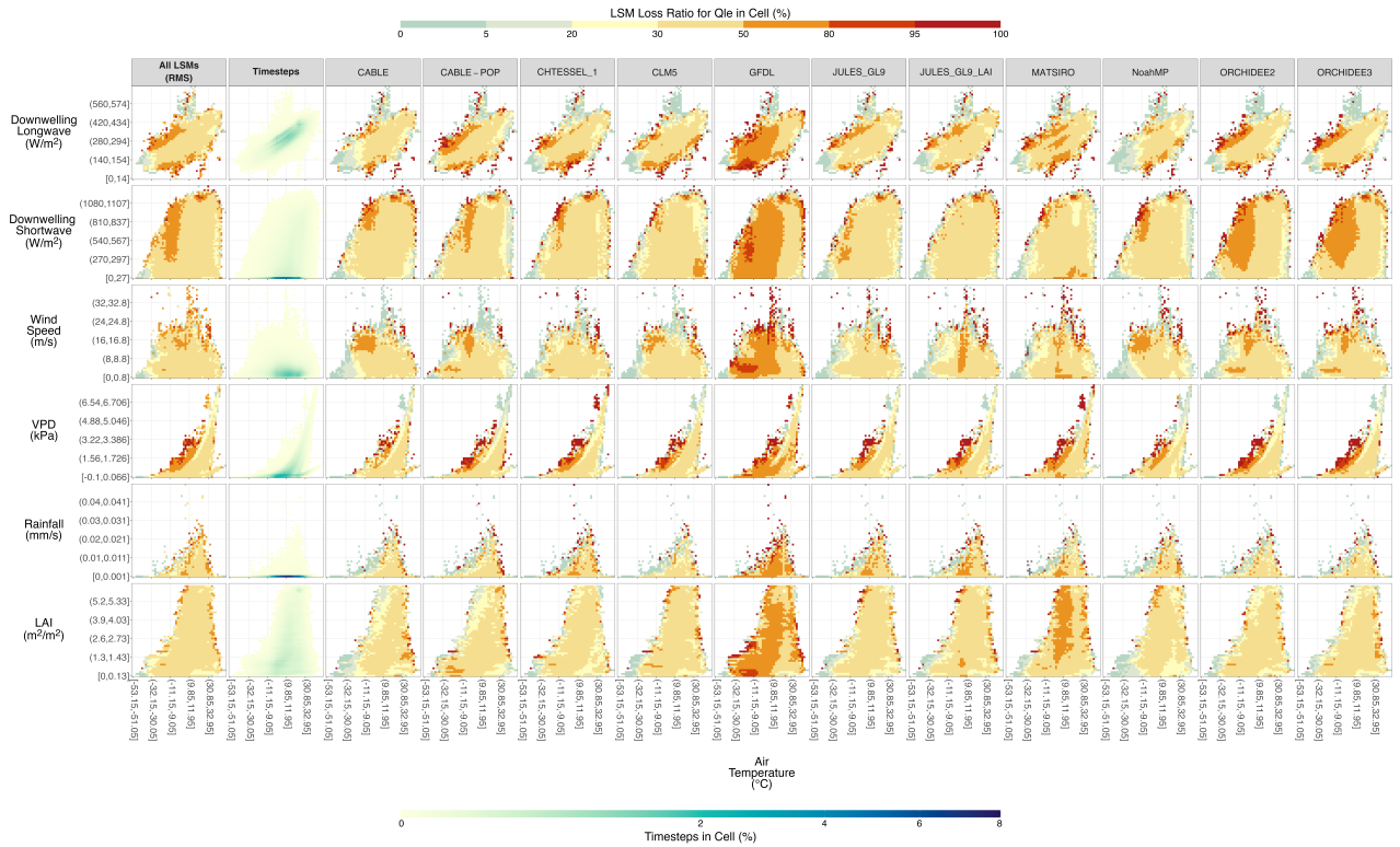
Figure 3. LSM Loss Ratio by Driving Variable and Model for Predicting Latent Heat Flux. The details are the same as Figure 2 but for predictions of the Qle flux.
