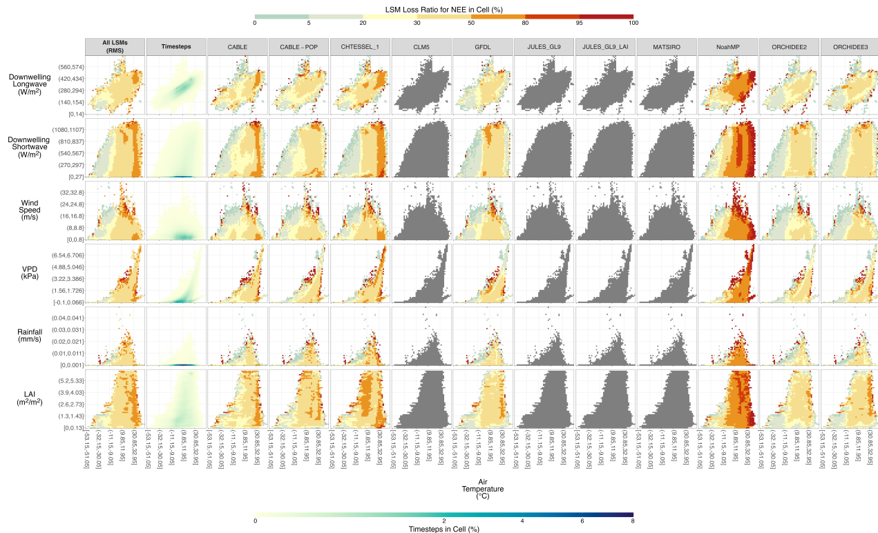
Figure 4. LSM Loss Ratio by Driving Variable and Model for Predicting Net Ecosystem Exchange. The details are the same as Figure 2 but for predictions of the NEE flux. Note that greyed out LSMs did not provide half-hourly NEE outputs to the PLUMBER2 experiment.
