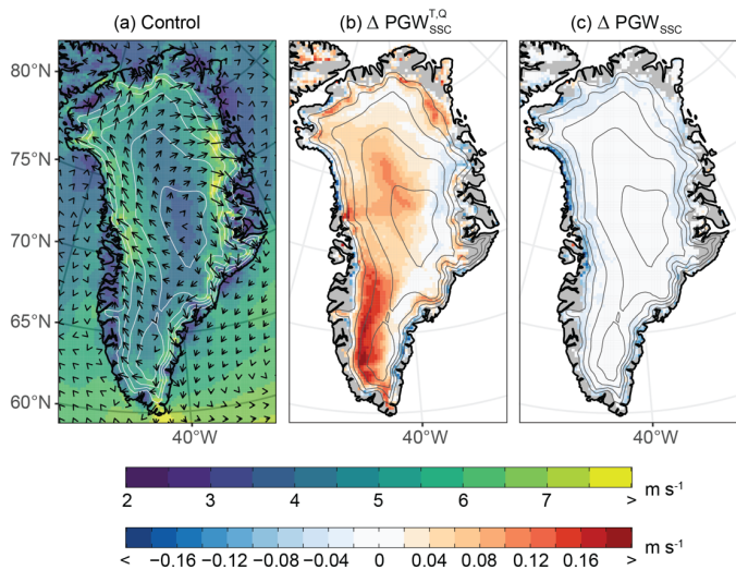
81 82 Figure 8: Melt season katabatic wind field under contrasting thermodynamic background conditions. (a) 2000–2019 long-term mean 83 Jun–Aug 10 m wind speed (shading) and direction (vectors). (b) Difference in 10 m wind speed between PGW_{SSC}^{T,Q} and the control. (c) 84 Difference in the 10 m wind speed between PGW_{SSC} and the control. \Delta = PGW - \text{Control} . Contour interval: 500 m. Range: 1000–3000 m. 85
