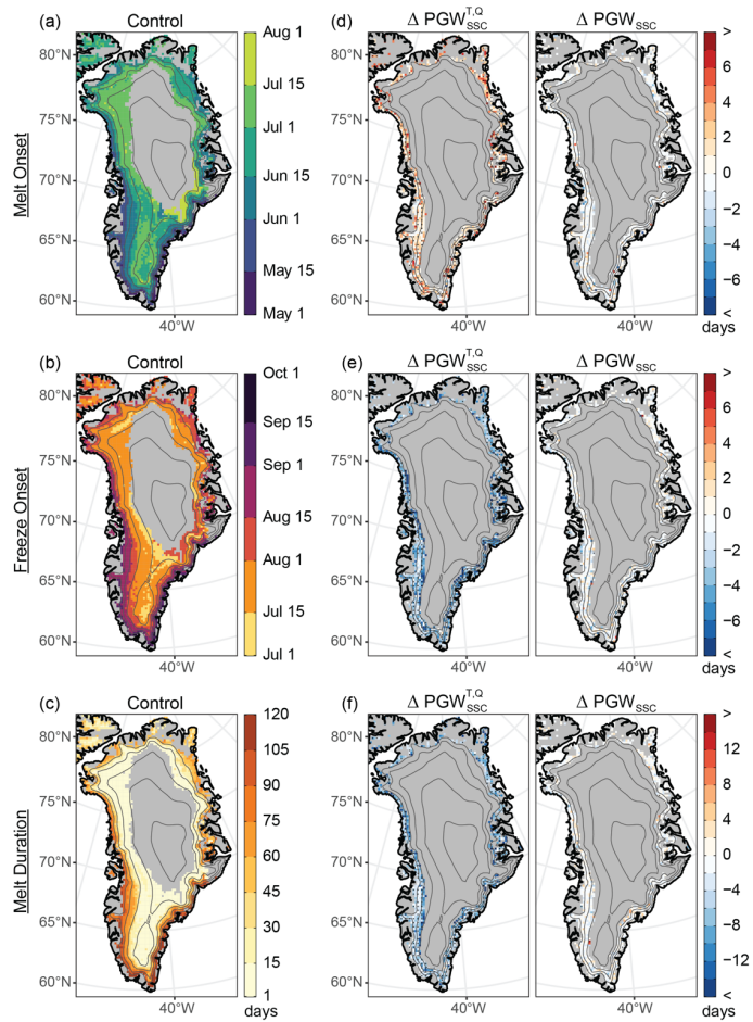
.52 .53 Figure 10. The impact of thermodynamic change on melt timing. The observed median date of (a) melt onset, (b) freeze onset and (c) .54 median melt season duration for the control simulation alongside (d–f) the difference between the PGW simulations ( PGW_{SSC}^{T,Q} , left; .55 PGW_{SSC} , right) and the control ( \Delta = PGW - \text{Control} ) for each metric as organized by row and labeled on the left. Stippling indicates .56 differences that are statistically significant at the 95% confidence level. Contour interval: 500 m. Range: 1000–3000 m.
