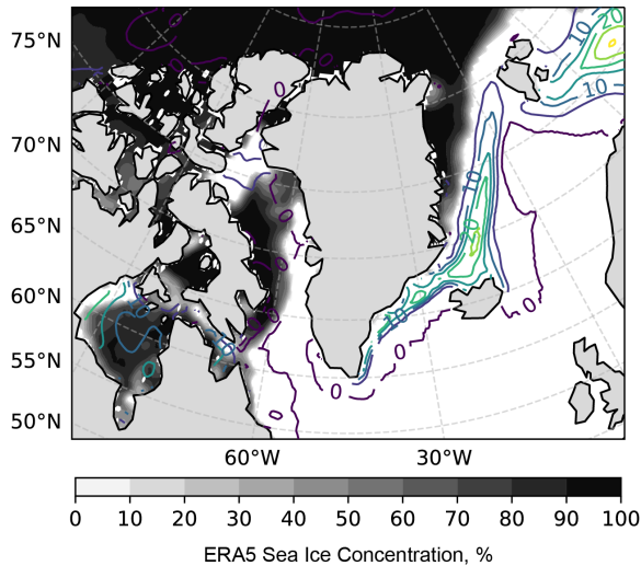
31 Figure 3. Sea ice representation. Comparison of observed sea ice concentration on June 15, 2018 (shading) and the corresponding CESM- 32 LE climate perturbation signal (contours, 5% interval). 33
