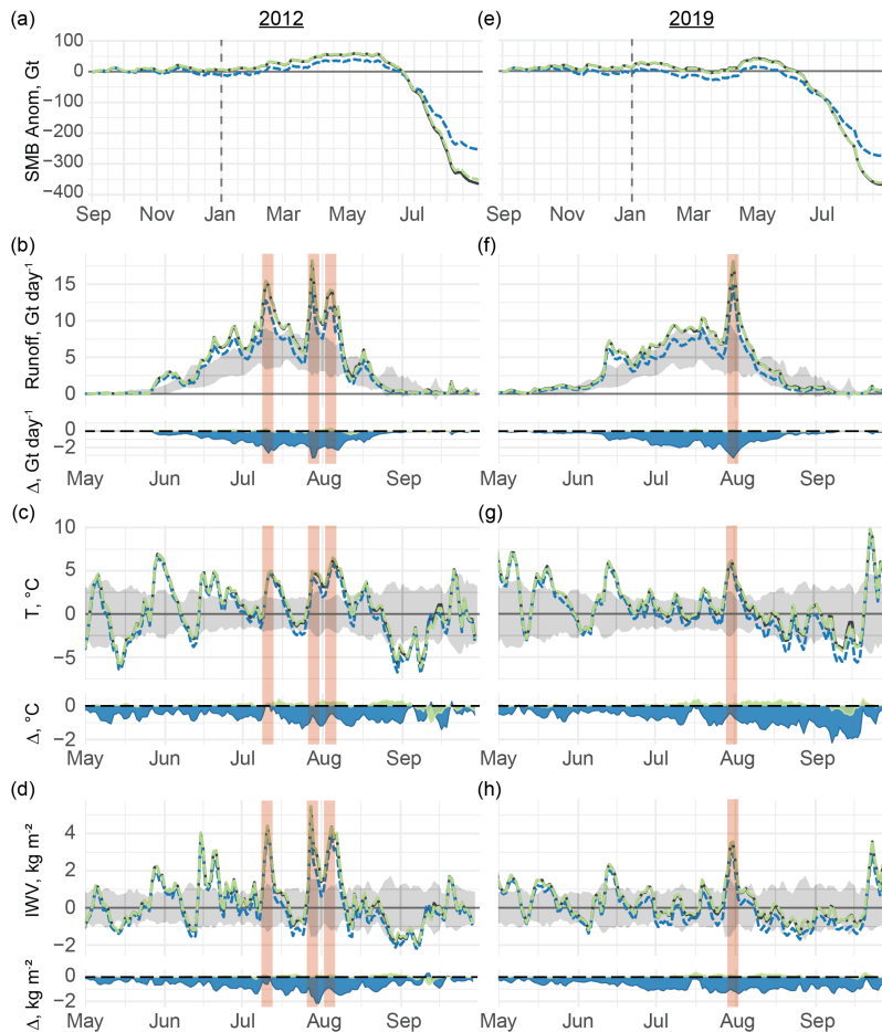
.92 Figure 11. Thermodynamic contribution to surface mass loss during years of exceptional melt. Panels show (a, e) the cumulative SMB .93 anomaly spanning the Sep–Aug hydrological year alongside (b, f) total daily meltwater runoff, (c, g) mean daily near-surface air temperature .94 anomaly, and (d, h) mean daily integrated water vapor anomaly during the exceptional melt years of (a–d) 2012 and (e–h) 2019. In all panels,
