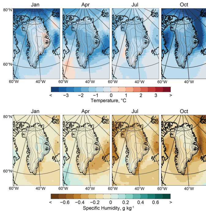
.18 Figure 2. Climate change perturbation fields. Perturbation fields derived from CESM-LE for surface air temperature (top row) and specific .19 humidity (bottom row) shown for a selection of months equally spaced throughout the year as labeled at the top of each panel. Perturbation .20 fields shown for the lowest model level after vertically interpolating to the same ECMWF L137 hybrid sigma-pressure levels as the .21 ERA5 boundary conditions. Contour interval: 500 m. Range: 1000–3000 m.
