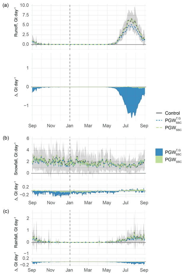
32 Figure 6. Seasonal evolution of the SMB under contrasting thermodynamic background conditions. Panels depict the seasonal 33 progression of three principal SEB components: (a) Surface runoff, (b) snowfall, (c) rainfall. Top portion of each panel shows 2000–2019 34 long-term daily mean totals of each SMB component throughout the melt season for the control (gray), PGW_{SSC}^{T,Q} (blue dashed), and PGW_{SSC} 35 (green dashed) simulations. Time series represent the spatially integrated sum of a given variable over the entire ice mask. Gray shading 36 shows the 1\sigma range about the mean for the control simulation. Bottom portion shows the difference between each PGW simulation ( PGW_{SSC}^{T,Q} , 37 blue; PGW_{SSC} , green) and the control ( \Delta = PGW - \text{Control} ). The scale of the y-axis on the bottom portion is kept constant across all panels 38 to facilitate comparison between SMB terms.
