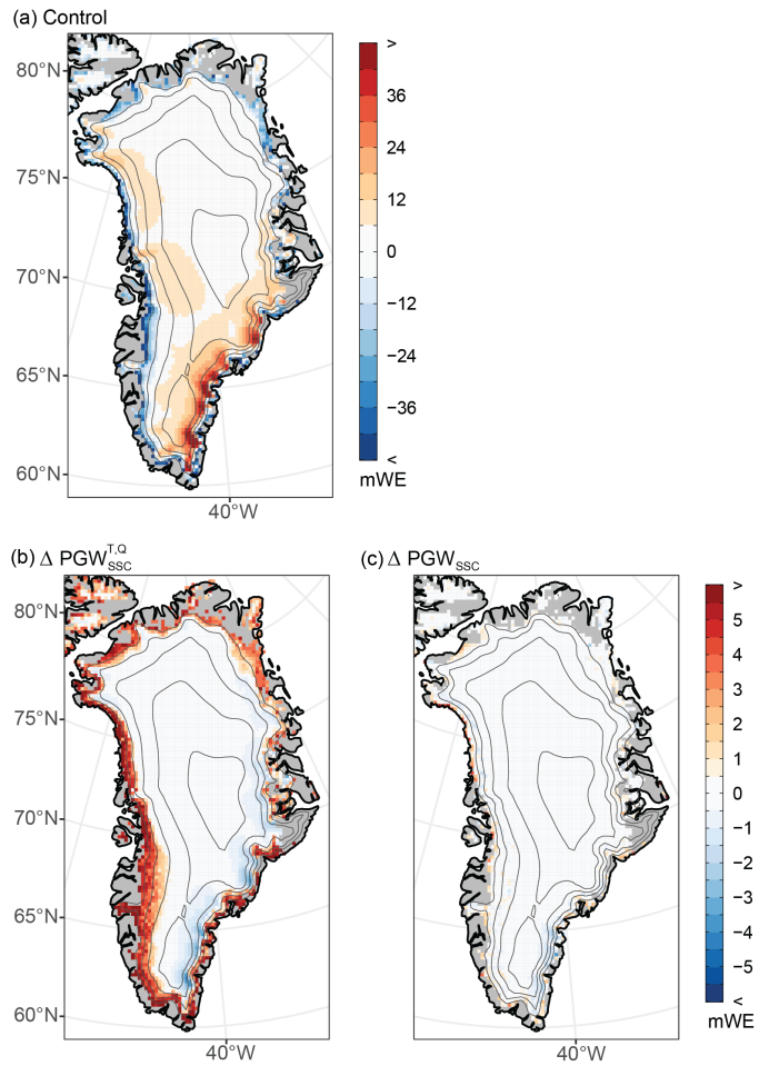
.90 Figure 5. Spatial distribution of SMB change under contrasting thermodynamic background conditions. (a) The cumulative SMB .91 anomaly over the full study period of 2000–2019 as represented by the control simulation. (b) PGW_{SSC}^{T,Q} cumulative SMB minus the control. .92 (c) PGW_{SSC} cumulative SMB minus the control. Contour interval: 500 m. Range: 1000–3000 m. .93
