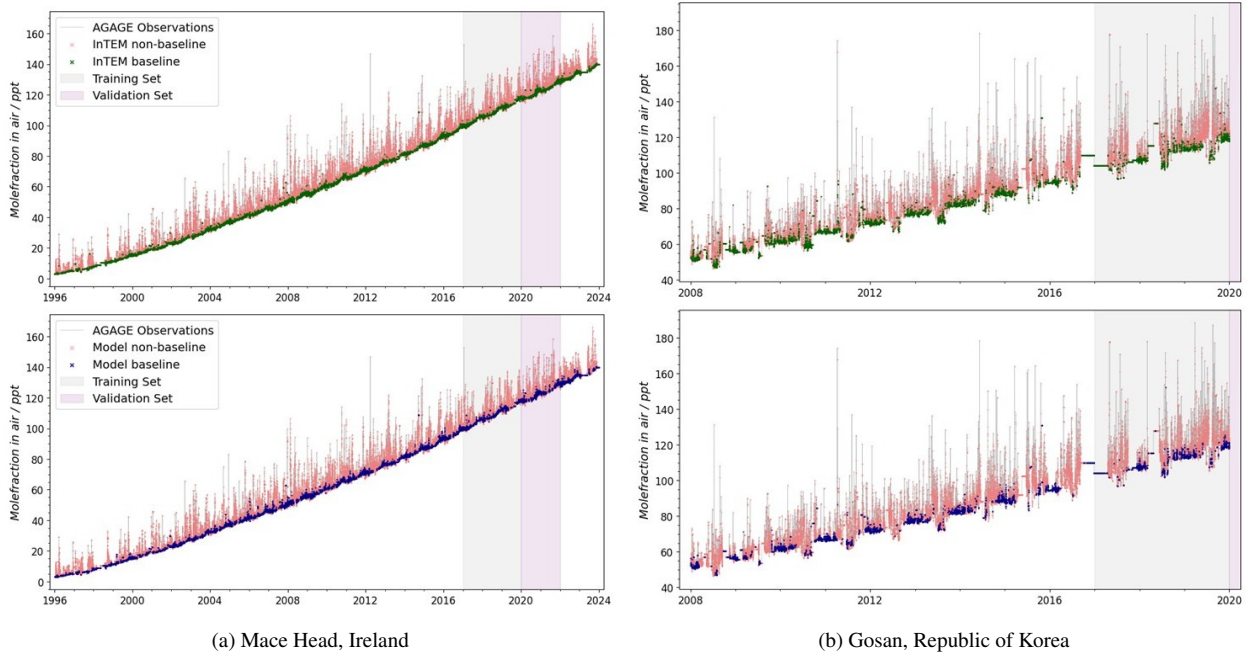
Figure 1. Measurement time series for HFC-134a ( \text{CH}_2\text{FCF}_3 ) at a) Mace Head, Ireland, and b) Gosan, Republic of Korea. The observations are shown as crosses and coloured according to the baseline/non-baseline label. The top panels show the measurements identified as baseline using the NAME/InTEM footprint-based filtering approach with no statistical filtering applied (green), and the bottom panels show the data points classified by the MLP algorithm presented here to be baselines (blue). The three-year training period is shown as grey shading and the two validation years are indicated by purple shading.
