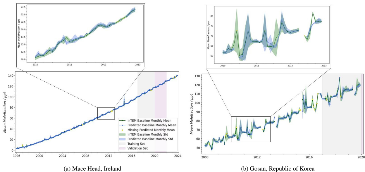
Figure 4. Baseline monthly means for HFC-134a at a) Mace Head, Ireland; b) Gosan, Republic of Korea. The NAME/InTEM baseline-derived values are represented by the green line, with associated 1\sigma variability within each month shown as green shading. The blue line shows the monthly means of data points that the MLP model classified as representative of baseline conditions. The 1\sigma variability within the model predicted monthly means is shown as blue shading. A subset of the dataset is shown in more detail in the top panels. Missing months are shown by yellow dots, and arise when a given month has no observations predicted as baseline by the model.
