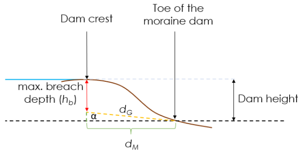
105 Figure 2. Estimating max. breach depth of a moraine-dammed lake. (A) shows a schematic picture of a moraine-dammed lake with 110 key terms. (B) shows how maximum breach depth is estimated for lakes with known bathymetry and (C) shows how maximum breach depth is estimated for lakes with unknown bathymetry.
