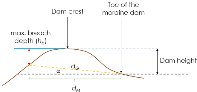
105 Figure 2. Estimating max. breach depth of a moraine-dammed lake. (A) shows a schematic picture of a moraine-dammed lake with 110 key terms. (B) shows how maximum breach depth is estimated for lakes with known bathymetry and (C) shows how maximum breach depth is estimated for lakes with unknown bathymetry.
