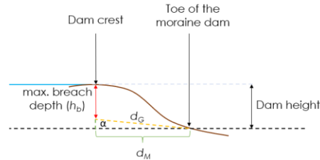
(C) Unknown bathymetry
