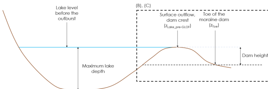
(B) Known bathymetry
