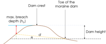
(A) Schematic picture of a moraine-dammed lake
