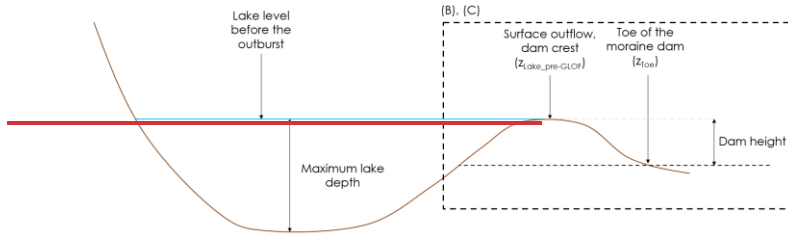
(B) Known bathymetry
