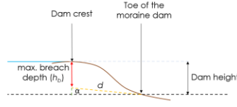
(A) Schematic picture of a moraine-dammed lake
