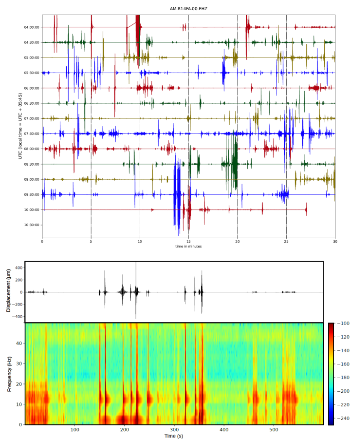
Figure 3: Seismometer recordings during exhibition activities (top) and jumping tests (bottom).
