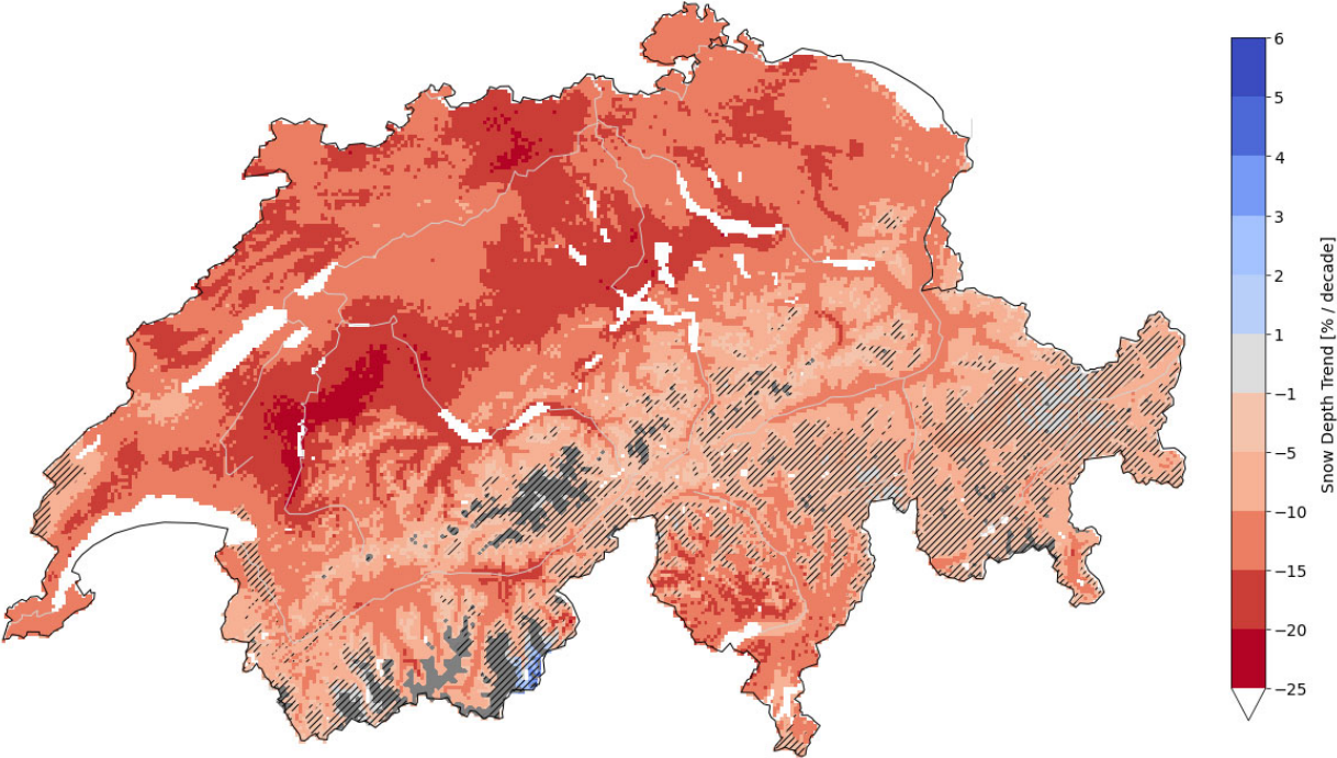
Figure S98: Relative trends of yearly mean snow depth (%/decade) for the period 1962 - 2023 based on Theil-Sen slopes for each 1-km grid point of the OSHD-CLQM model in Switzerland. Water bodies appear white, elevations above 3000 m are colored in grey and non-hatched areas indicate significant trends at 95% confidence level, p < 0.05 .
