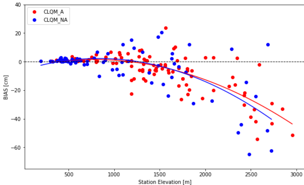
315 Figure 6: BIAS of yearly mean snow depth [cm] vs elevation [m] for the comparison of assimilated (red) and non-assimilated (blue) stations value with respect to the OSHD-CLQM model. The curves are polynomials fits of second degree.
