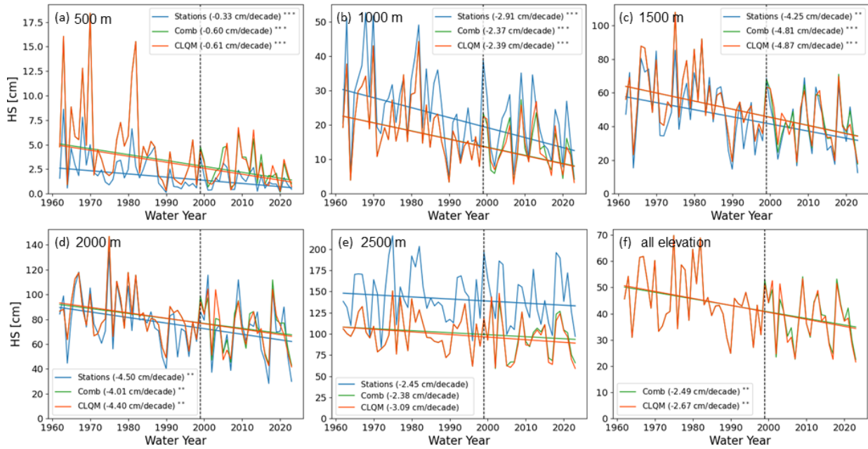
Figure 7: Trends of yearly snow depth [cm / decade] calculated using Theil-Sen slopes for the OSHD-CLQM and the combined model data series (OSHD-Comb), as well as for station measurements for the five elevation bands: (a) 500, (b) 1000, (c) 1500, (d) 2000, (e) 2500 m, and (f) all elevation (0-3000 m). Significance is indicated by * p < 0.05 ; ** p < 0.01 ; *** p < 0.001 . The dashed line indicates the year 1999, before which the yearly values of OSHD-CLQM and OSHD-Comb are the same.
