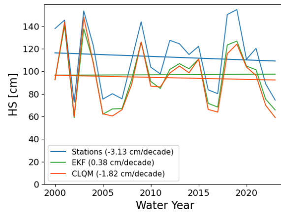
Figure S76: Trends of yearly snow depth [cm / decade] calculated using Thiel-Sen slopes for the OSHD-CLQM and the OSHD-EKF, as well as for station measurements (mean of 16 stations) for the highest elevation band (2500 m). Possible significance is indicated with * p < 0.05 ; ** p < 0.01 ; *** p < 0.001 .
