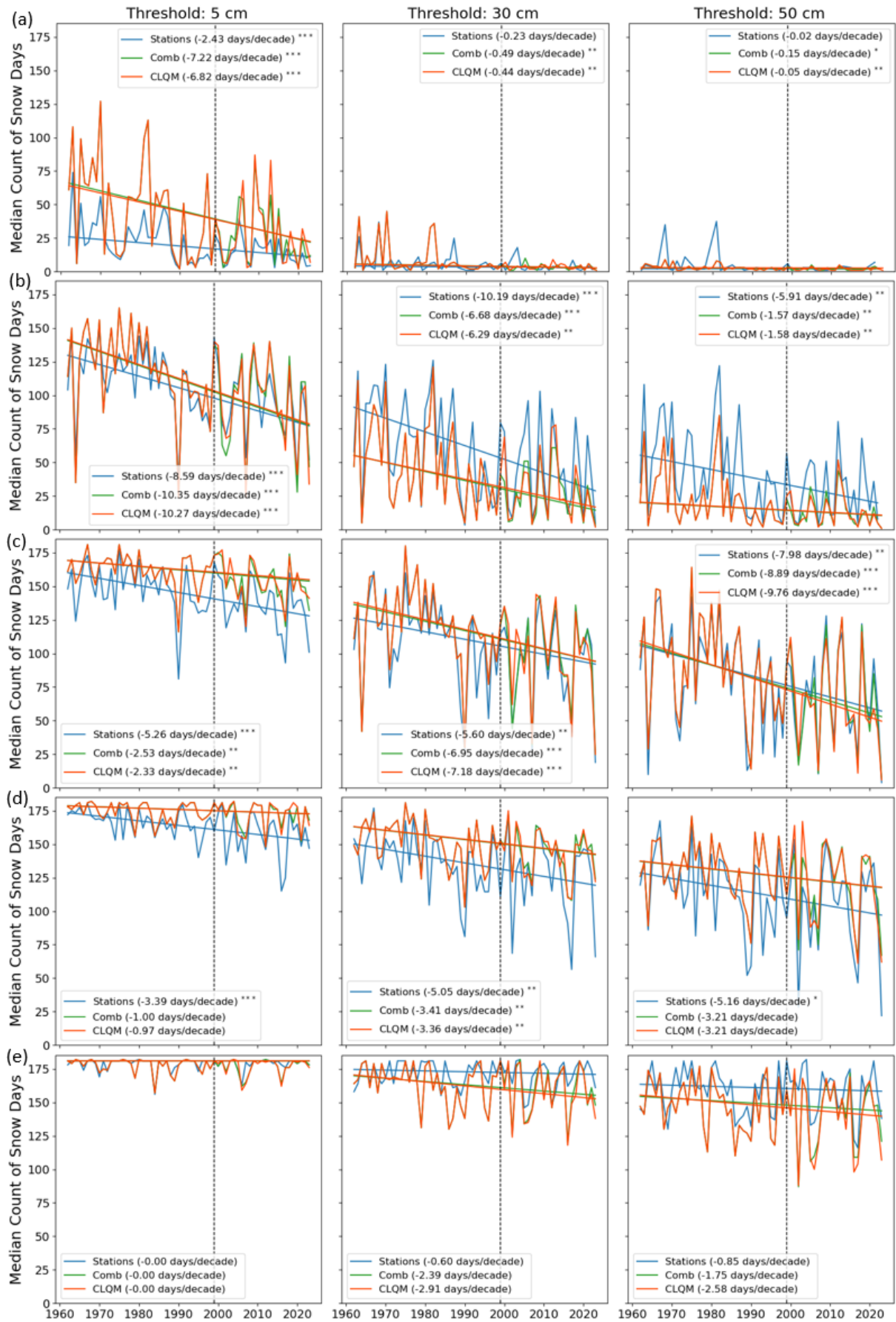
Figure S87: Trends of median snow days for three different thresholds (5,30, 50 cm) using Theil-Sen-slope regression for OSHD-CLQM and OSHD-comb, as well as stations across five elevation bands: (a) 500, (b) 1000, (c) 1500, (d) 2000, and (e) 2500 m. Significance is indicated with * p < 0.05 ; ** p < 0.01 ; *** p < 0.001 . The dashed line indicates the year 1999, before which the yearly values of OSHD-CLQM and OSHD-comb are the same.
