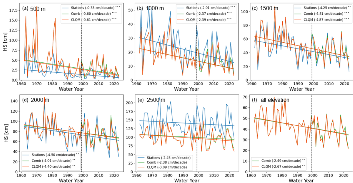
335 Figure 7: Trends of yearly snow depth[cm / decade] calculated using Theil-Sen slopes for the OSHD-CLQM and the combined model data series (OSHD-Comb), as well as for station measurements for the five elevation bands: (a) 500, (b) 1000, (c) 1500, (d) 2000, (e) 2500 m and (f) entire Switzerland (0-3000 m). Significance is indicated with * p < 0.05 ; ** p < 0.01 ; *** p < 0.001 . The dashed line indicates the year 1999, before which the yearly values of OSHD-CLQM and OSHD-comb are the same. 340
