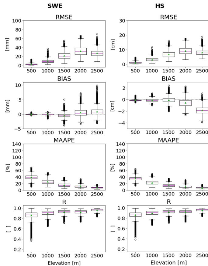
Figure 4: Score comparison between models OSHD-CLQM and OSHD-EKF ('reference') on a yearly resolution at respective elevation bands (m) for SWE (left) and HS (right). Boxplots were generated from these performance scores to illustrate the distribution, outliers, mean (green triangle) and median (purple line). The box reflects the 50 % of data between the lower quartile and upper quartile. The whiskers extend from the boxes' edges and correspond to 1.5 IQR. Outliers are represented as individual dots.
