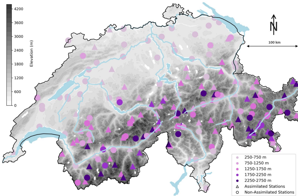
115 Figure 2: Map of Switzerland with the elevation of the individual grid points and the distribution of stations used to validate the gridded datasets. Stations are colored by elevation band; assimilated stations (OSHD-EKF) are shown as triangles and non-assimilated stations as circles.
