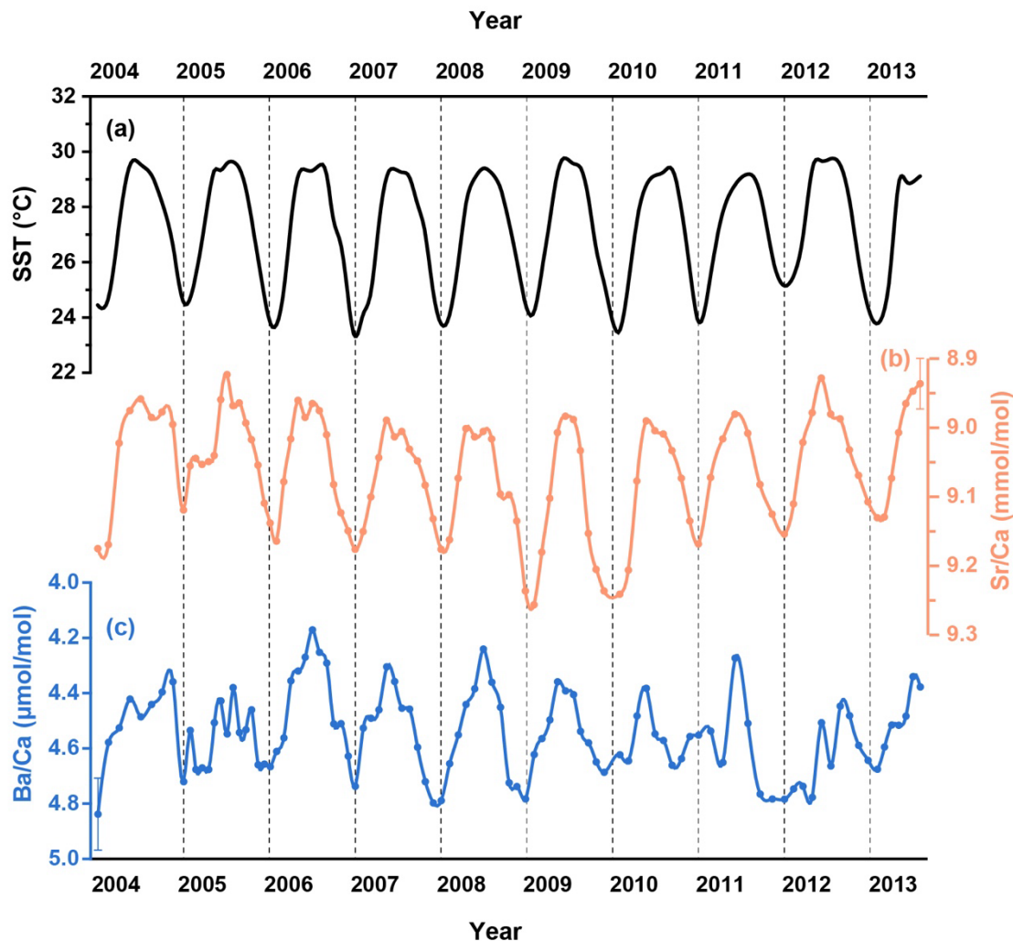
155 Figure 2: (a) The U.K. Meteorological Office Hadley Centre Global Sea Ice and Sea Surface Temperature (HadISST, Rayner et al., 2013). Monthly resolved coral geochemical data for (b) Sr/Ca and (c) Ba/Ca from the coral samples in the South China Sea.
