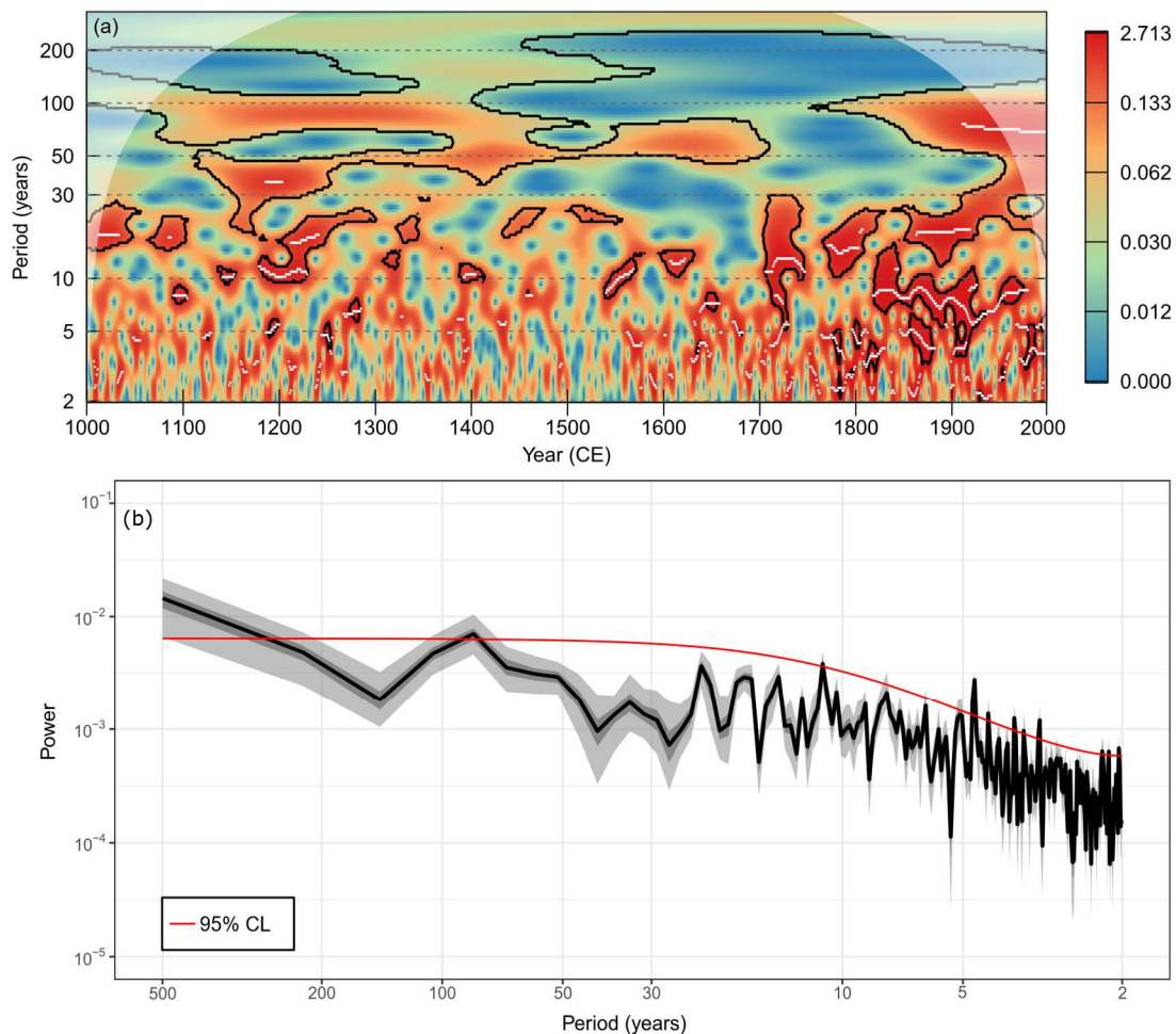
Figure 6. (a) Wavelet decomposition of the NAO reconstruction from 1000–2000 CE. Color contours are scaled by power quantiles. Black contours bound statistically significant power ( p < 0.05 ) and white curves show ridges (power maxima). White envelope shows the region where padding may influence estimates. (b) The multi-taper method spectral decomposition for the NAO reconstruction. Red line shows 95% confidence level based on an AR(1) null. Grey shading shows ensemble range.
