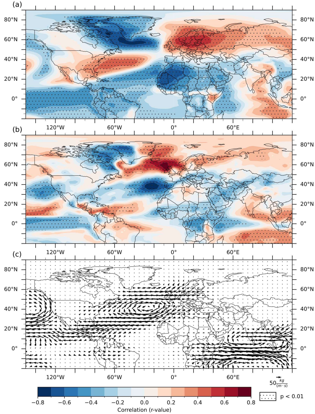
Figure 5. Winter NAO ILME correlations (color contours) with iLME winter surface air temperature, precipitation amount, and composite IVT from 1823–2000 CE. Stippling denotes p < 0.01 . (a) NAO ILME correlation with winter surface air temperature. (b) NAO ILME correlation with winter precipitation amount. (c) Difference between winter IVT during positive and negative winter NAO ILME years, defined as NAO ILME greater or less than one standard deviation from the mean, respectively, over the period 1823–2000 CE.
