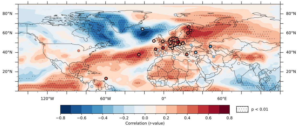
Figure 4. Winter \text{NAO}_{\text{iLME}} correlations (color contours) with \text{iLME} winter \delta^{18}\text{O}_{\text{precip}} from 1823–2000 CE. Stippling denotes p < 0.01 . Symbols show GNIP stations with \geq 10 winters colored by \delta^{18}\text{O}_{\text{precip}} correlations with \text{NAO}_{\text{vinther}} , bold symbols show significant ( p < 0.1 ) correlations.
