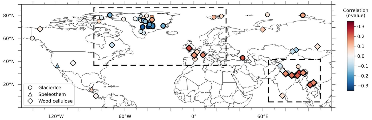
Figure 1. Map of Iso2k records included in the analysis. Shapes correspond to archive type and colors denote the Pearson’s r -value of each record with NAO_{Vinther} (1823–2000 CE). Bold outlines signify significant correlation ( p < 0.1 ). Regional subsets used for validation are indicated by dashed boxes over Greenland and southeast Asia.
