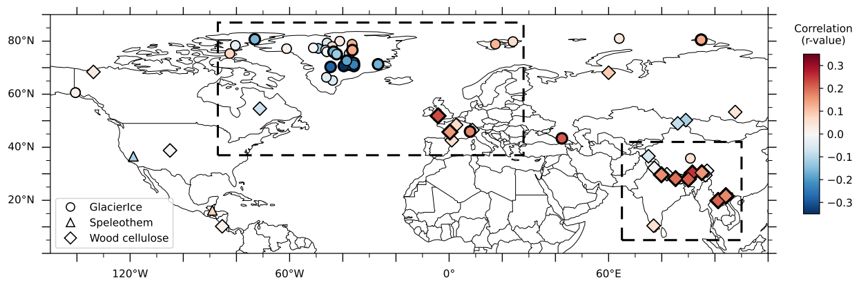
Figure 1. Map of Iso2k records included in the analysis. Shapes correspond to archive type and colors denote the Pearson’s r -value of each record with NAO_{Vinter} (1823–2000 CE). Bold outlines signify significant correlation ( p < 0.1 ). Regional subsets used for validation are indicated by dashed boxes over Greenland and southeast Asia.
