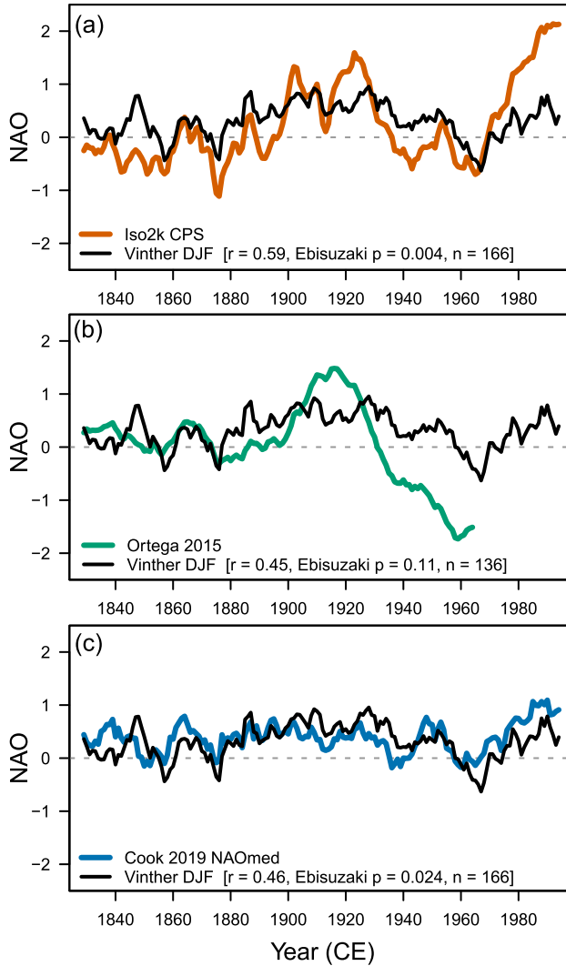
Figure 7. Decadally smoothed NAO reconstructions during the observational period compared with the decadal smoothed \text{NAO}_{\text{Vinther}} index (black lines). Series were smoothed using an 11-year centered running mean. (a) Iso2k CPS reconstruction (this study; orange) vs. \text{NAO}_{\text{Vinther}} . (b) Ortega et al. (2015) calibration constrained median (teal) vs. \text{NAO}_{\text{Vinther}} . (c) Cook et al. (2019) \text{NAO}_{\text{med}} (blue) vs. \text{NAO}_{\text{Vinther}} .
