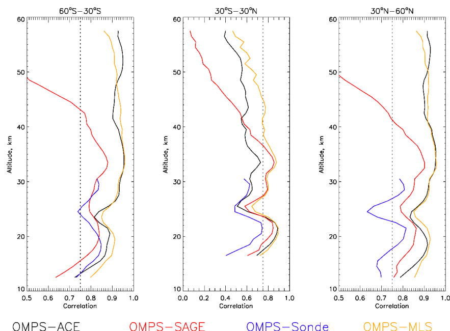
OMPS-ACE OMPS-SAGE OMPS-Sonde OMPS-MLS Figure 5: Vertical profiles of correlation coefficients between OMPS LP and matched correlative observations for 3 wide latitude bands.
