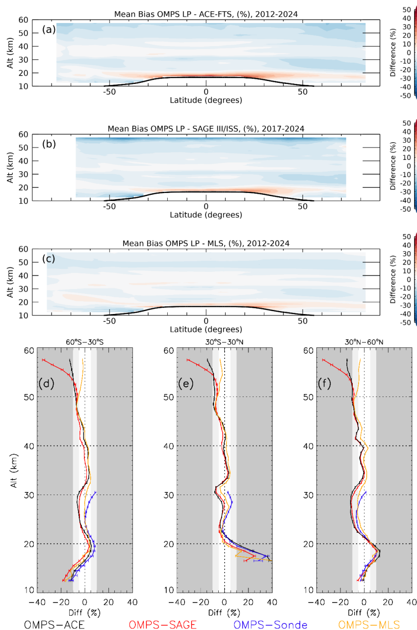
Figure 4: Profile differences between OMPS LP and matched correlative satellite and ground-based observations. Panels (a-c) show zonal mean differences between OMPS LP and ACE-FTS, OMPS LP and SAGE III/ISS and OMPS LP and MLS on a 5° latitude grid. Panels (d-f) show mean profile differences between OMPS LP and ACE-FTS (black), OMPS LP and SAGE III/ISS, OMPS LP and ozonesondes (blue) and OMPS LP and MLS (Orange) for 3 wide latitude bands, the horizontal bars show 2 times the standard error of the mean (SEM), the white area indicates differences less than 5%, the light grey area 5-10% and the dark grey area represents differences greater than 10%, only data above the tropopause are shown.
