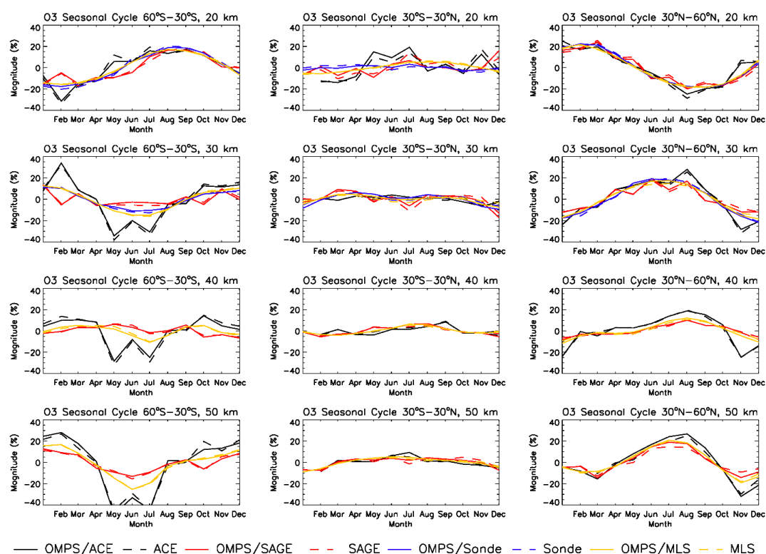
Figure 6: Seasonal cycle in co-located OMPS LP (solid lines) and correlative observations (dashed lines) calculated as monthly mean deviations from the long-term annual mean in % calculated for each instrument independently. OMPS seasonal cycles are calculated using a sub-set of matching profiles for each correlative instrument.
