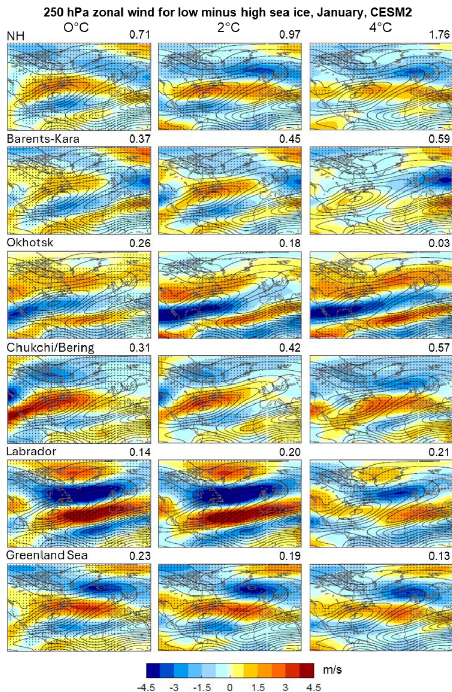
365 Figure 7: Mean difference in January zonal wind at 250 hPa for low minus high January sea ice states in a selection of Arctic seas for a selection of global warming levels (ranging from 0 to 4 °C) in CESM2. Positive values denote an increase in wind blowing from west to east (or a slowdown from East to West). Also shown with contours is the climatological mean zonal wind over the preindustrial period, which indicates the average position of the North Atlantic jet stream (contour interval 5 m s -1 , negative contours are dashed). Stippling indicates a significant zonal wind difference between low and high sea ice states using a t-test (p<0.05). 370 Numbers in the top right corners indicate the change in sea ice area between low and high sea ice states in units of a million km 2 .
