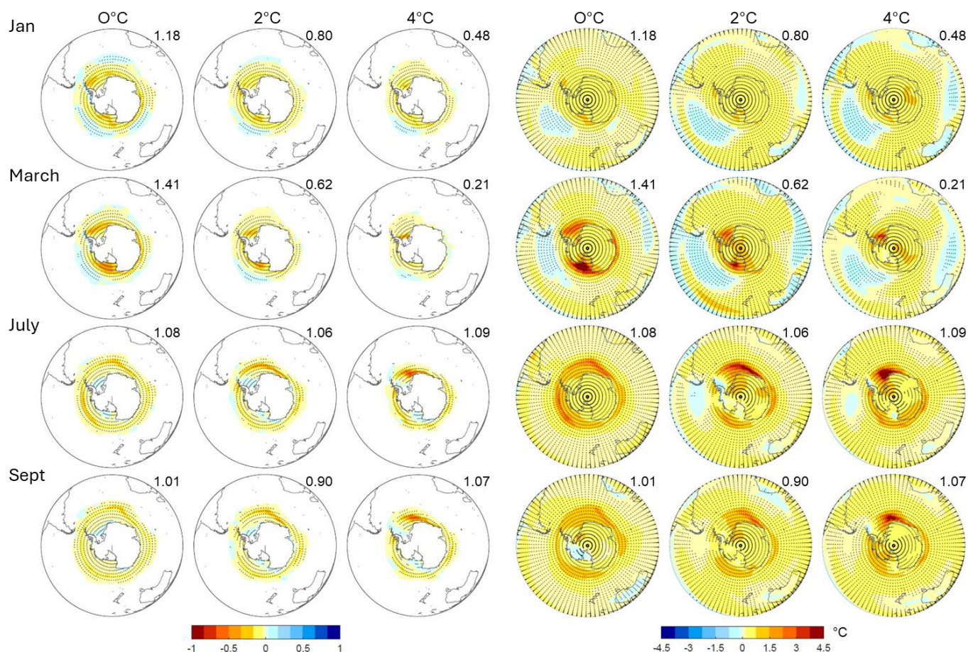
405 Figure 8: Left side- difference in sea ice fraction between low and high Antarctic sea ice states for selected global warming levels (ranging from 0 to 4°C) and months (January, March, July, September). Right side- the same but for surface air temperature. Stippling denotes significance with a t-test ( p>0.05 ). Numbers in the top right corners indicate the change in sea ice area between low and high sea ice states in units of a million km 2 .
