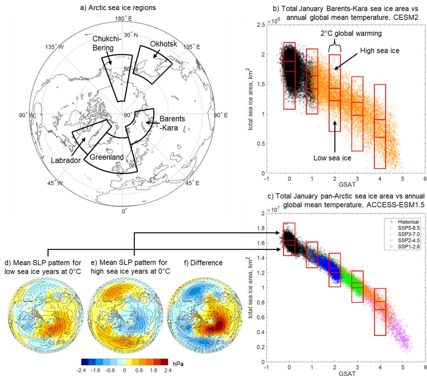
Figure 1: a) The Arctic sea ice regions considered (see also Table 1) b) Interannual variability in January sea ice area for the Barents-Kara Seas vs annual mean global surface air temperature (GSAT, °C) for the CESM2 large ensemble for 1850-2100. Red boxes illustrate the selection of points for “high” (>70 th percentile) and “low” (<30 th percentile) sea ice areas for different global warming levels. c) as for panel b) but for January pan-Arctic sea ice for ACCESS-ESM1.5 and the inclusion of multiple scenarios. Panels d) and e) show the average sea level pressure anomalies relative to the preindustrial period (1850-1900) associated with low and high January pan-Arctic sea ice states respectively at the example warming level of 0°C for ACCESS-ESM1.5. Panel f) shows the difference between panels d) and e), and thus the average difference in SLP for winters with low sea ice minus those with high sea ice. Stippling in f) indicates a significant difference of the mean of SLP between low and high sea ice states using a t-test ( p < 0.05 ). Contours in d-e) indicate climatological mean SLP over the preindustrial period (1850-1900), with a contour interval of 4 hPa, with contours 1014 hPa or less dashed.
