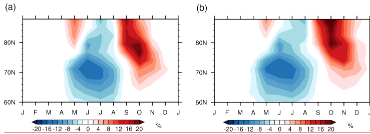
Figure 10: Difference in zonal and monthly mean low-level cloud amount cover between LIG and PI: (%); (a) \Delta LIGvALIGvS; and (b) \Delta LIGvCLIGvL.
