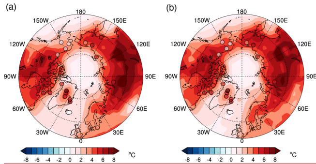
Figure 8: Comparison of simulations with proxies for the ALIG (LIG – PI) summer SAT difference (June-July-August): (a) ALIGvS; and (b) ALIGvL. The circles represent proxy data from Guarino and Sime (2022).
