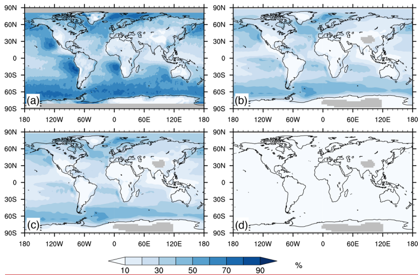
Figure A3: Annual mean low-level cloud cover (%): (a) CALIPSO-GOCCP (Chepfer et al., 2010); (b) P1vS; (c) P1vL; and (d) the difference between 1880-1899 in the historical and preindustrial simulations of Yoshimori et al. (2018). Note that low-level cloud cover is diagnosed assuming the maximum-random overlap for clouds with optical depth \tau > 0.3 as a standard model output.
