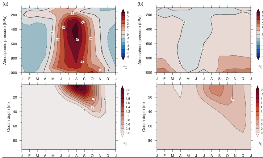
470 Figure 12: Temperature anomalies in the atmosphere and the upper ocean (°C): (a) \Delta LIGvS; and (b) \Delta LIGvL - \Delta LIGvS. The regional average is taken for the Arctic Ocean (60-90°N).
