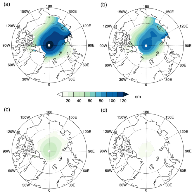
360 Figure 7: September sea-ice thickness (cm) in the Arctic: (a) PH+APIvS ; (b) PH+CP1vL ; (c) LG+ALIGvS ; and (d) LG+CLIGvL .
