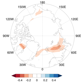
Figure A2: Difference in September sea ice concentration between 1880-1899 in the historical and preindustrial simulations of Yoshimori et al. (2018).
