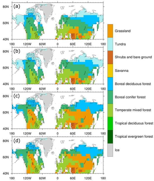
Figure 3: Simulated vegetation distribution: (a) PIvAPIvS ; (b) PIvCPIvL ; (c) LIGvALIGvS ; and (d) LIGvCLIGvL . These maps show the dominant (most frequent) vegetation type in each grid cell over the last 100 years of the integrations. Note that each grid cell is occupied by a single vegetation type, although this may vary over time.
