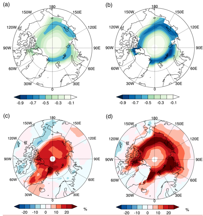
460 Figure 11: Changes in sea ice concentration and low-level cloud amount cover for \Delta LIGv-ALIGvS : (a) August ice concentration; (b) September ice concentration; (c) September cloud amount cover (%); and (d) October cloud amount cover (%).
