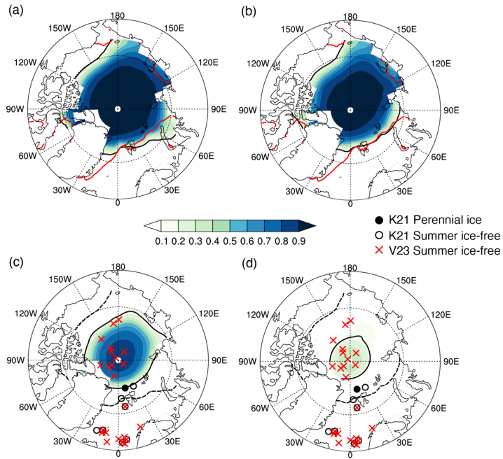
Figure 6: September sea-ice concentration in the Arctic: (a) PI+APIvS ; (b) PI+CP1vL ; (c) LIG+ALIGvS ; and (d) LIG+CLIGvL . In (a) and (b), black lines denote the simulated boundaries for the ice concentration of 0.15, while red lines denote the observed ones (HadISST2, by Titchner and Rayner, 2014). In (c) and (d), black solid lines denote the simulated boundaries for the ice concentration of 0.15, while black dashed lines denote those in the corresponding preindustrial simulations. The year-round ice cover (solid circles) and summer ice-free conditions (empty circles) suggested by proxies are also plotted: Black symbols for proxy data from Kageyama et al. (2021), and summer ice-free conditions (red symbols for cross marks) from Vermassen et al. (2023) are also plotted. Note that only proxies claimed as good chronological control are shown for Kageyama et al. (2021), and whether the data from Vermassen et al. (2023) actually represent LIG has been questioned, as stated in the Introduction.
