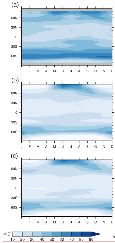
730 Figure A4: Seasonal progression of low-level cloud cover (%): (a) CALIPSO-GOCCP (Chepfer et al., 2010); (b) PIVS; and (c) PIVL. Note that low-level cloud cover is diagnosed assuming the maximum-random overlap for clouds with optical depth \tau > 0.3 as a standard model output.
