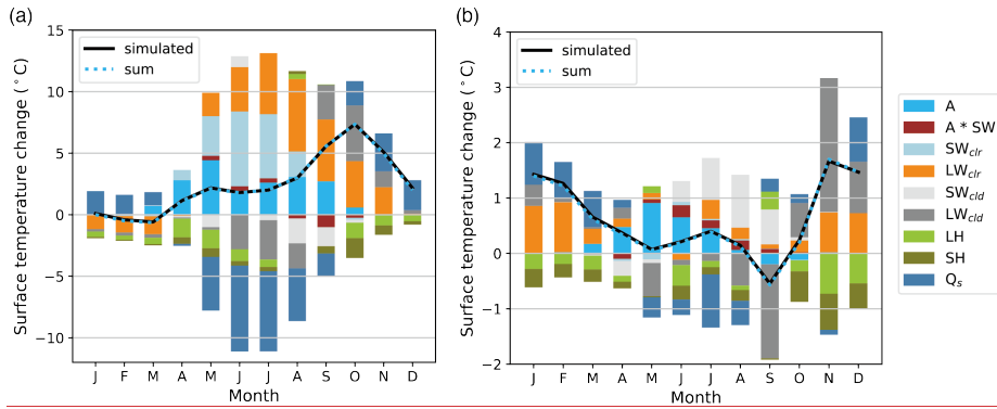
435 Figure 9: Attribution of Arctic Ocean (60-90°N) surface temperature difference to feedback components (°C): (a) \Delta LIGvA ( LIGvA - Piv ) and (b) \Delta LIGvCLIGvL - \Delta LIGvALIGvS . Please see Table 54 for the description of each feedback component. In the stacked vertical bars, the positive contributions are shown above the zero horizontal line and the negative ones below. The solid black polygonal line denotes simulation, and the dashed blue line represents the sum of the diagnosed partial temperature differences, i.e., the cumulative value of the vertical bars.
