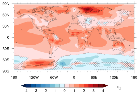
Figure 2: Difference in annual mean surface air temperature SAT between PivCPIvL and PivAPIvS (°C). Grid cells for which the difference is not statistically significant at the 5% level are hatched.
