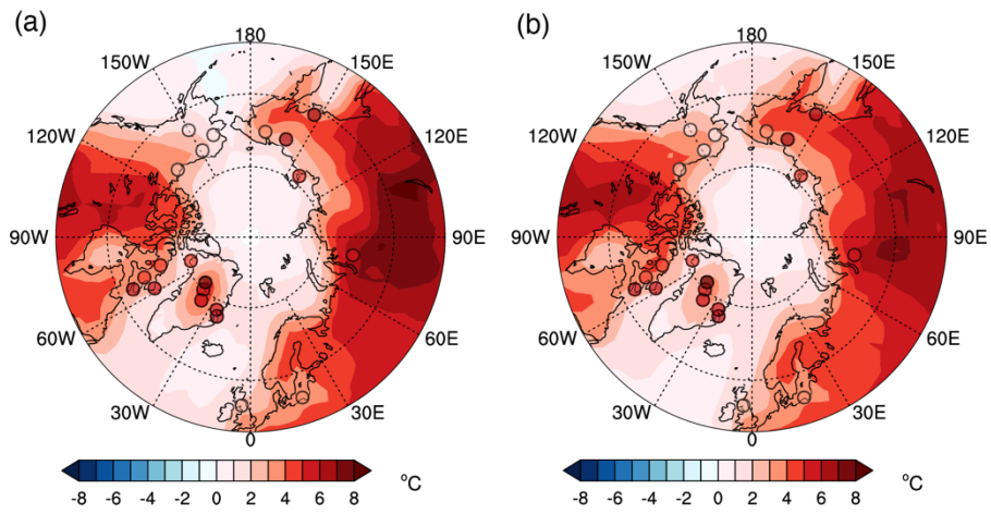
60 Figure S6: Comparison of simulations with proxies for the \Delta LIG (LIG-PI) summer SAT difference (June-July-August): (a) \Delta LIGfS; and (b) \Delta LIGfL. The circles represent proxy data from Guarino and Sime (2022). This figure corresponds to Fig. 8 of the main text, which presents the MIROC4mV results.
