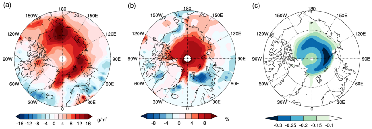
430 Figure 13: Difference between \Delta LIGvL and \Delta LIGvS: (a) liquid water path (from October to December) ( \text{g}/\text{m}^2 ); (b) low-level cloud cover (from October to December) (%); and (c) sea ice concentration (from September to November).
