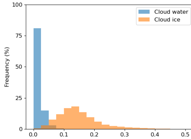
Figure S1: Histograms of the monthly mean autoconversion rate ( -1/L \cdot dL/dt ) of cloud particles with L being the cloud liquid or solid water content for PIVS using MIROC4mV. The data represent grid points below the 680 hPa level in the Arctic. The unit of the horizontal axis is 1/hour. The vertical axis is the fraction of the total number of grid cells points. The results for PIVL, LIGvS, and LIGvL are qualitatively similar.
