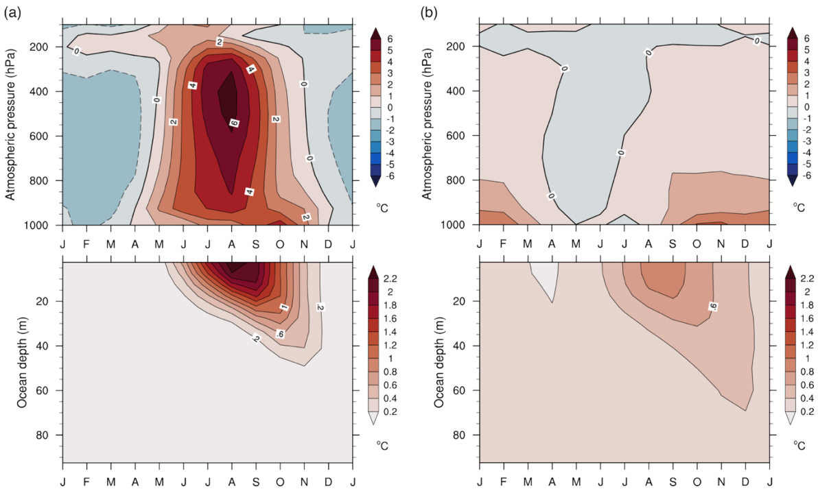
Figure 12: Temperature anomalies in the atmosphere and the upper ocean (°C): (a) \Delta\text{LIGvS} ; and (b) \Delta\text{LIGvL} - \Delta\text{LIGvS} . The regional average is taken for the Arctic Ocean (60-90°N).
