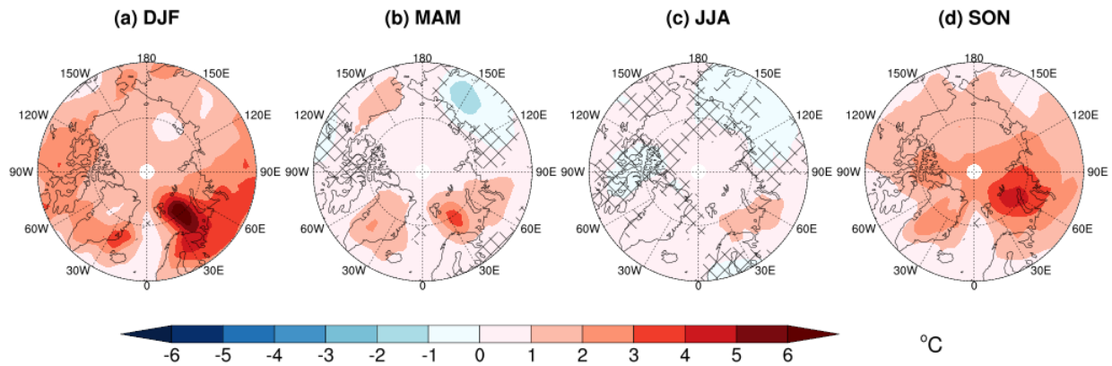
35 Figure S2: Difference in surface air temperature between PIvL and PIvS (°C): (a) December-January-February; (b) March-April-May; (c) June-July-August; and (d) September-October-November. Grid cells for which the difference is not statistically significant at the 5% level are hatched.
