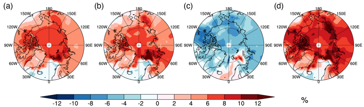
Figure A5: Difference in the annual mean low-level cloud cover (%): (a) PivL – PivS by MIROC4mV; (b) as (a) but reproduced by the AGCM (PivL_LL – PivS_SS); (c) AGCM with only the temperature-phase parameter swapped in (b) (PivL_SL – PivS_LS); and (d) AGCM with other cloud parameters swapped in (b) (PivL_LS – PivS_SL).
