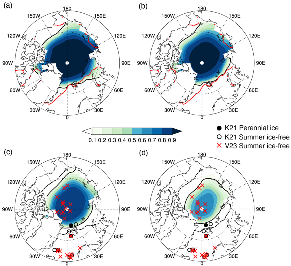
Figure S8: September sea-ice concentration in the Arctic: (a) PIfS; (b) PIfL; (c) LIGfS; and (d) LIGfL. In (a) and (b), black lines denote the simulated boundaries for the ice concentration of 0.15, while red lines denote the observed ones (HadISST2 by Titchner and Rayner, 2014). In (c) and (d), black solid lines denote the simulated boundaries for the ice concentration of 0.15, while black dashed lines denote those in the corresponding preindustrial simulations. The year-round ice cover (solid circles) and summer ice-free conditions (empty circles) suggested by proxy data from Kageyama et al. (2021), and summer ice-free conditions (red cross marks) from Vermassen et al. (2023) are also plotted. Note that only proxies claimed as good chronological control are shown for Kageyama et al. (2021), and whether the data from Vermassen et al. (2023) actually represent LIG has been questioned, as stated in the Introduction. This figure corresponds to Fig. 6 of the main text, which presents the MIROC4mV results.
