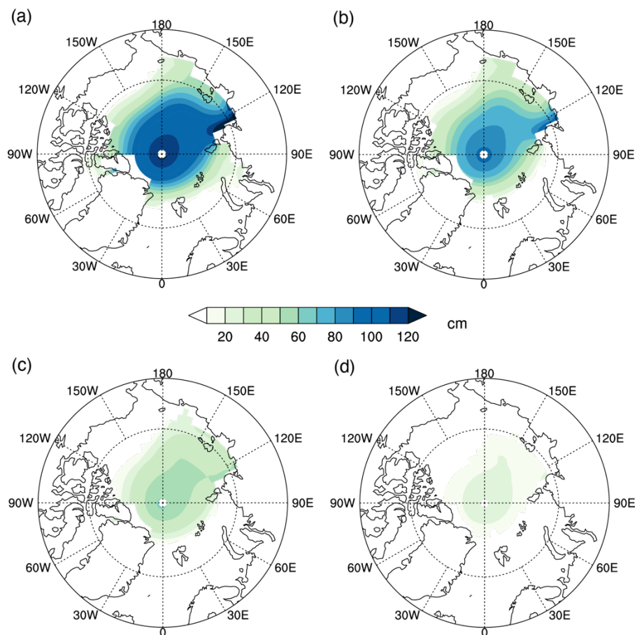
55 Figure S5: September sea-ice thickness (cm) in the Arctic with MIROC4m: (a) P1fS; (b) P1fL; (c) L1GfS; and (d) L1GfL. Note that grid cells where the ice concentration is less than 0.15 are not coloured. This figure corresponds to Fig. 7 of the main text, which presents the MIROC4mV results.
