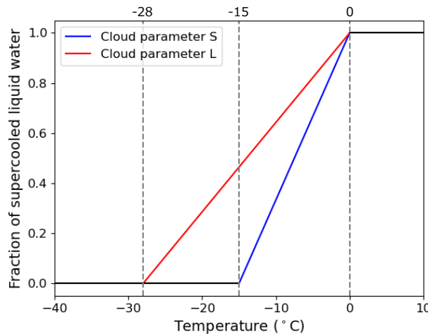
Figure 1: Fraction of supercooled liquid water in the two cloud-parameter sets S ( T_{ice} = -15^\circ\text{C} ) and L ( T_{ice} = -28^\circ\text{C} ). Vertical gray dashed lines indicate the temperature ranges within which solid and liquid phases coexist in cloud particles.
