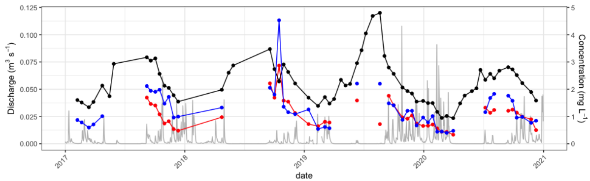
340 Figure 5. Stream discharge (grey), and water concentration of Fe (blue) and Pb x 200 (red) and C in DOC x 0.05 (black) from S1. Discharge shows daily averages of measurements made every 15 min, whereas concentrations in water were analysed from grab samples usually every 2-3 weeks during high flow and throughout 2019. Dots mark timing of sampling. Data points for Fe and Pb were removed when discharge <0.0001 ( m^3 s^{-1} ), which occurred during summer when the water level was too low to measure discharge, making calculation of export 345 impossible.
