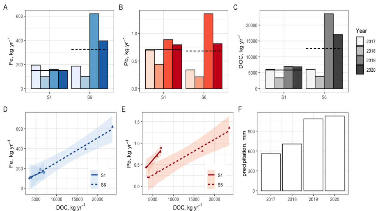
Figure 6. Annual export of DOC, Fe and Pb from Mycklemossen to Ersjön lake (S1) and from Ersjön (S6) in 2017 to 2020 (A-C) and the linear relationship between export of DOC and export of Fe and Pb (D and E). Horizontal lines in bar chart are means of the years 2017-2020 in S1 (solid line) and S6 (hatched line). Note differences in scale between plots. Annual precipitation for the years 2017-2020 (F).
