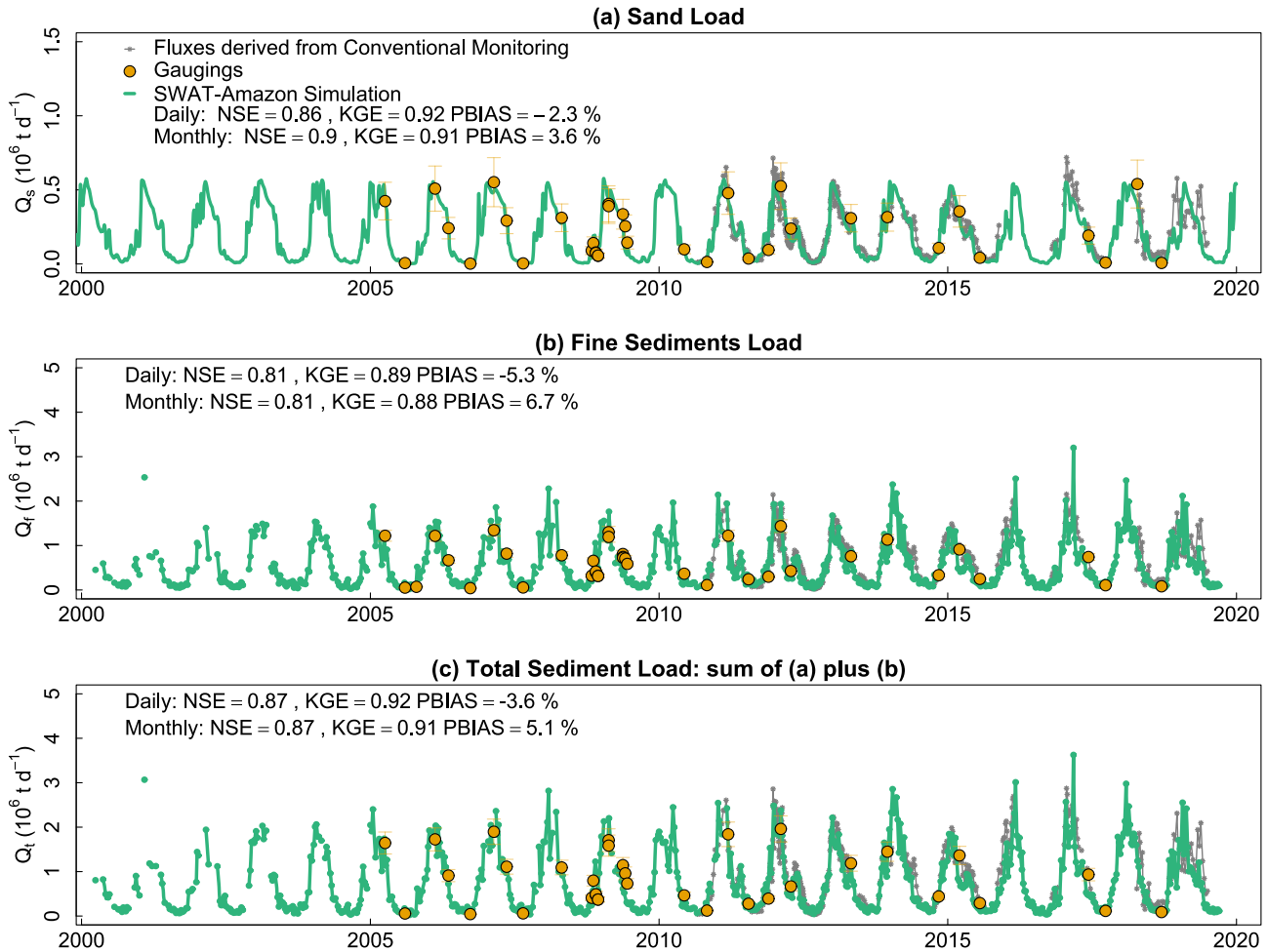
575 Figure 8: Integrated monitoring of sediment fluxes at the basin outlet. The gray line with stars shows observed sediment fluxes, the green line represents SWAT-Amazon simulations, and orange filled circles indicate gauged flux values.
