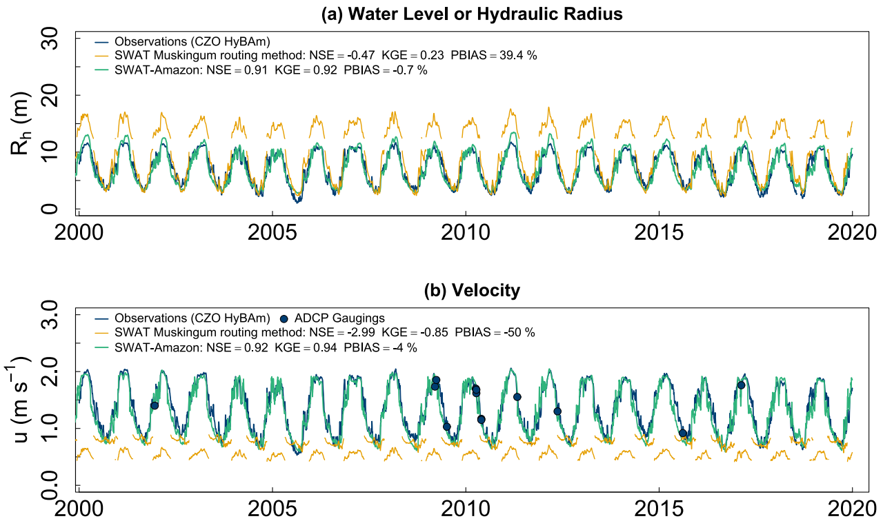
485 Figure 4: Example of (a) water levels and (b) velocities simulation at Pucallpa. Marine blue line: observations, orange line: best default SWAT simulation with Muskingum, green line: SWAT-Amazon simulation, blue filled circle: ADCP gauging values. Error bars, which were less than 3% for ADCP measurements, are not shown for clarity.
