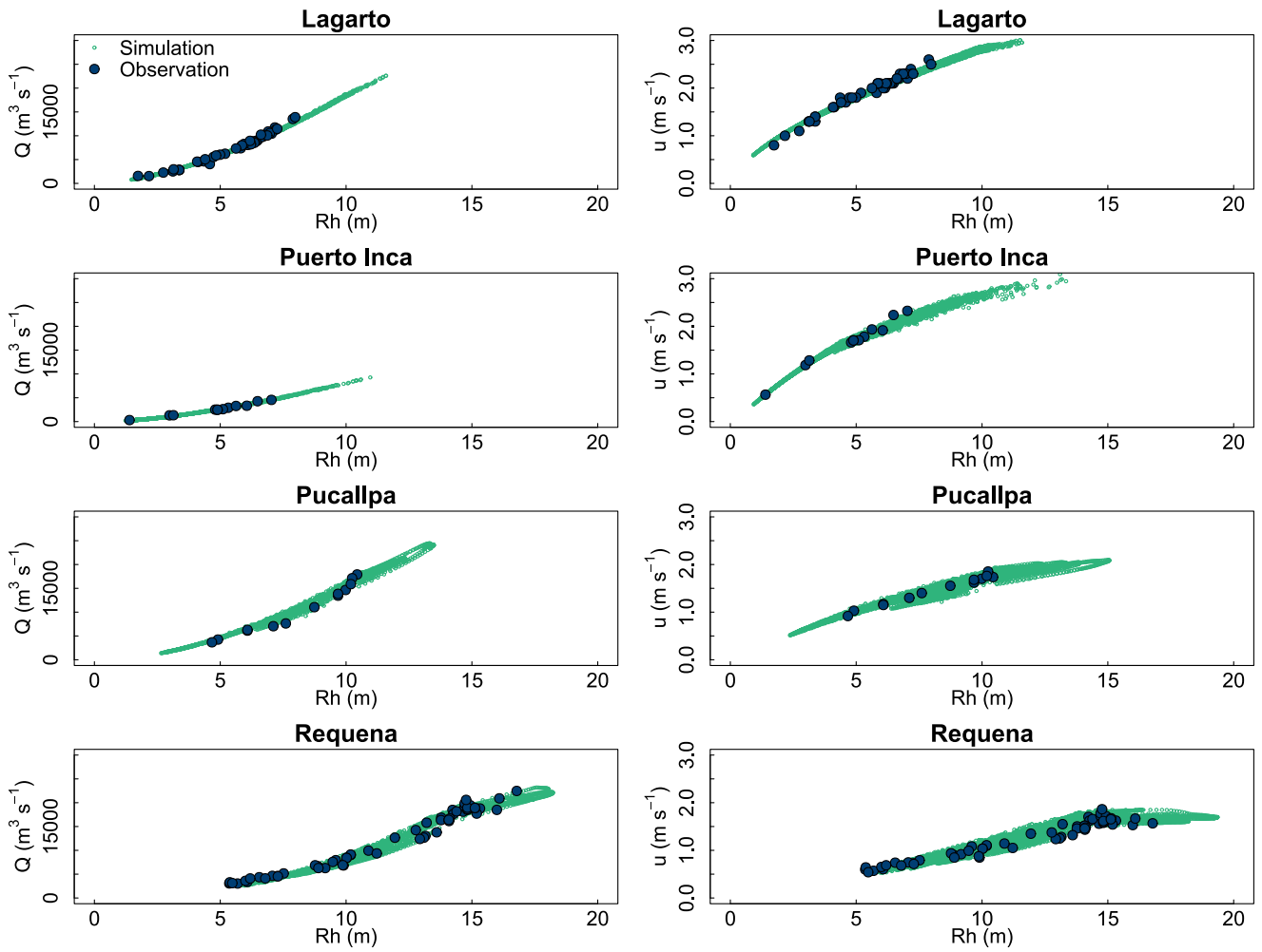
490 Figure 5: Rating curves between hydraulic radius ( R_h ) and discharge (left) or velocity (right). Green circles: SWAT-Amazon simulation, blue filled circles: ADCP measurements.
