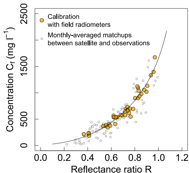
550 Figure 7: Relationship between fine sediment concentration ( C_f ) at the water surface and the ratio R of NIR to red reflectance. Orange dots represent calibration points, based on 42 field measurements in the Ucayali Basin, where reflectance was measured using a hyperspectral radiometer and fine sediment concentrations were measured at the water surface. Gray dots correspond to matchups between satellite-derived reflectance ratio and fine sediment concentrations monitored at gauging stations, averaged at a monthly time step.
