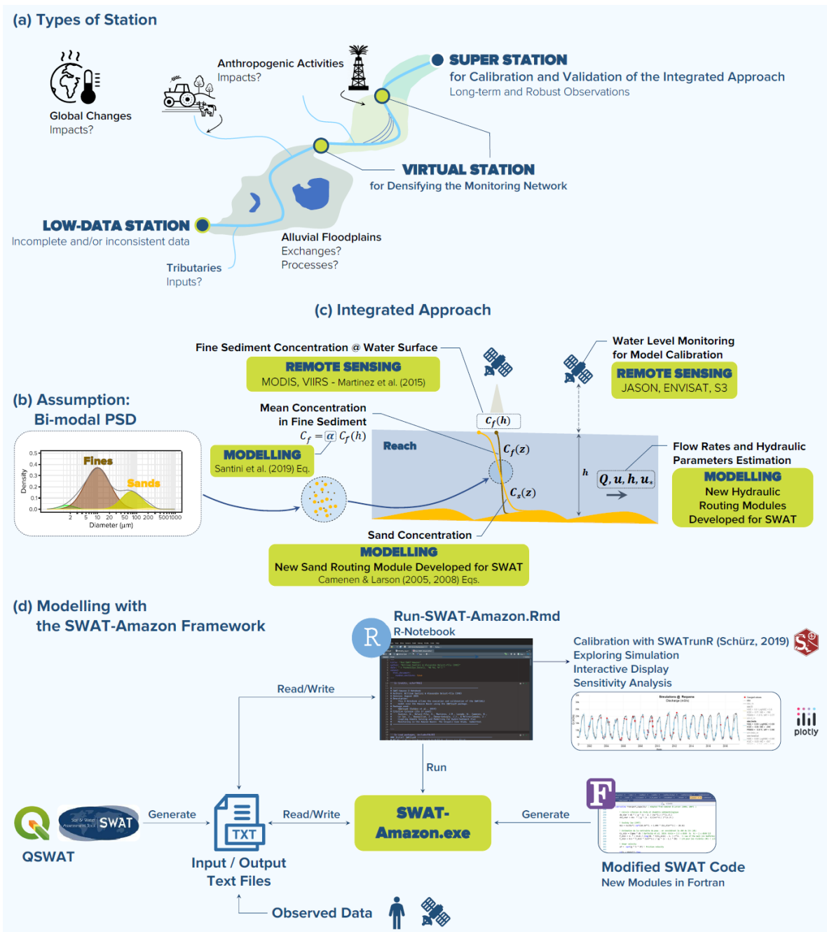
150 Figure 1: General schematic overview of the proposed methodology. Panels (a–c) illustrate the integrative approach. (a) Types of stations. (b) Typical bimodal particle size distribution (PSD) in the large Amazonian rivers, identifying two main size groups: 1- fine sediments that can be monitored by satellite but not modelled; 2- fine sands in graded suspension, invisible to satellites but whose transport capacity can be modelled. (c) Integrated approach combining remote sensing, modelling, and calibration campaigns. (d) SWAT-Arizona, a tailored version of the SWAT model for simulating water and sand fluxes. This modelling framework consists of a Fortran-based executable (SWAT-Arizona.exe) and an R notebook (Run-SWAT-Arizona.Rmd) used for model runs, simulation analysis, interactive visualization, sensitivity analysis and calibration with the SWATrunR package (Schürz et al., 2019). 155
