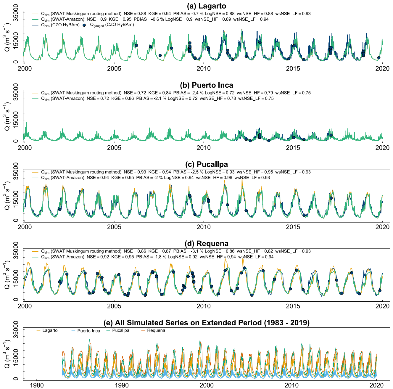
Figure 3: Water discharge simulations for the stations with gauging data (a) – (d) Observed discharge (marine blue) vs. simulated discharge using the default SWAT model (orange) and SWAT-Amazon (green) at a daily time step, with punctual ADCP gauging values (blue circles). (e) Full 37-year simulation (1983–2019) with SWAT-Amazon for the same station group.
