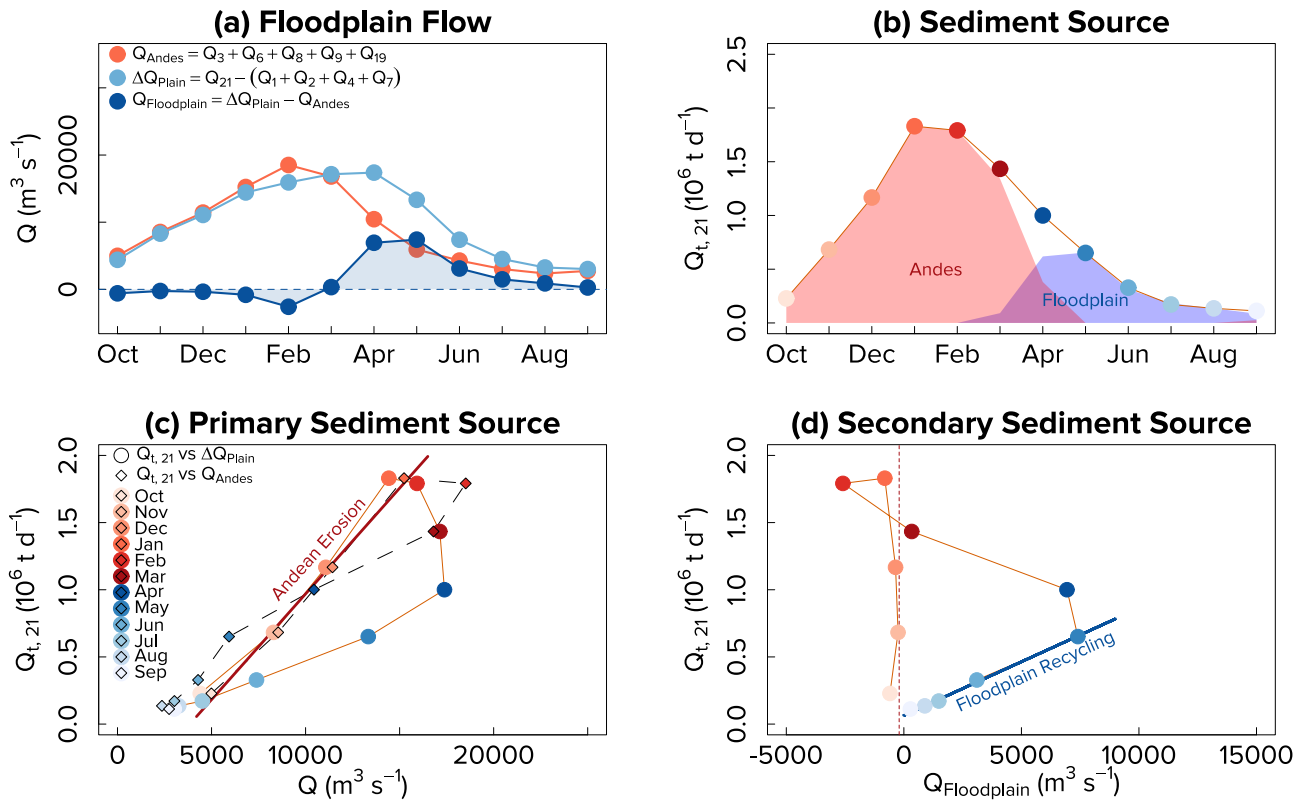
835 Figure 12: Identification of sediment sources at the interannual scale. (a) Water discharge components: Andean Basin outflow ( Q_{Andes} ), basin outlet discharge excluding lateral contributions ( \Delta Q_{plain} ) and floodplain flows ( Q_{Floodplain} ), all in \text{m}^3 \text{ s}^{-1} . (b) Decomposition of total sediment flux at the basin outlet Q_{t,21} ( 10^6 \text{ t d}^{-1} ) by sediment sources: red for Andean erosion, blue for floodplain recycling. (c) Relationship between Q_{t,21} and \Delta Q_{plain} (circles) and Q_{Andes} (diamonds). The red regression line represents the relationship between Q_{Andes} and Q_{t,21} during rising limb months (d) Relationship between Q_{t,21} and Q_{Floodplain} . The blue regression line illustrates the relationship between Q_{Andes} and Q_{t,21} during recession months.
