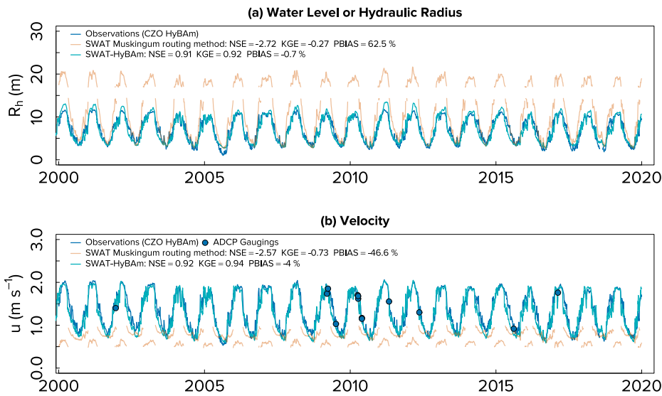
Figure 4: Example of (a) water levels and (b) velocities simulation at Pucallpa. Marine blue line: observations, orange line: best default SWAT simulation with Muskingum, green line: SWAT-Amazon simulation, blue filled circle: ADCP gauging values. Error bars, which were less than 3% for ADCP measurements, are not shown for clarity.
