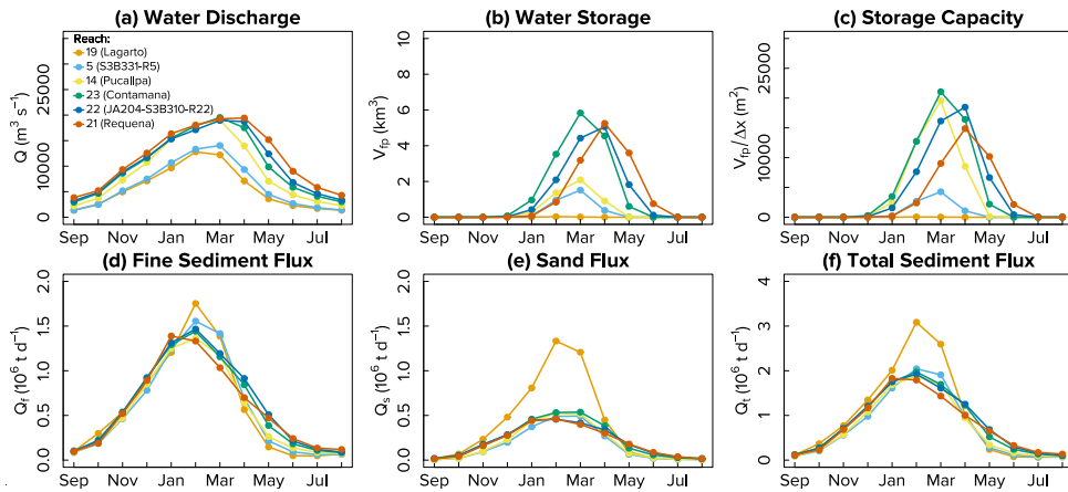
880 Figure 11: Interannual water (1983–2019) and sediment (2000–2019) balances along the Ucayali River. Lines show interannual monthly means and shaded bands represent the 5th–95th percentile envelope of the behavioural GLUE ensemble (2500 runs). (a) Water Discharge (b) Floodplain water storage ( V_{fp} ) in \text{km}^3 . (c) Normalization of V_{fp} by the reach's length ( \Delta x ) for cross-sub-basin comparison. (d) Fines suspended sediments. (e) Suspended sand fraction. (f) Total suspended sediment load. See Supplement S12 for full uncertainty propagation details.
