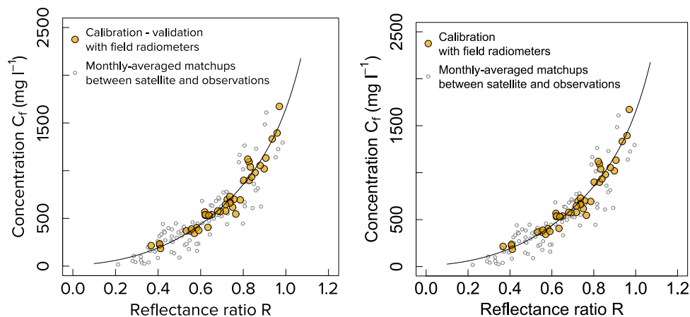
Figure 7: Relationship between fine sediment concentration ( C_f ) at the water surface and the ratio R of NIR to red reflectance. Orange dots represent calibration and validation points, based on 42 field measurements in the Ucayali Basin, where reflectance was measured using a hyperspectral radiometer and fine sediment concentrations were measured at the water surface. Gray dots correspond to matchups between satellite-derived reflectance ratio and fine sediment concentrations monitored at gauging stations, averaged at a monthly time step.
