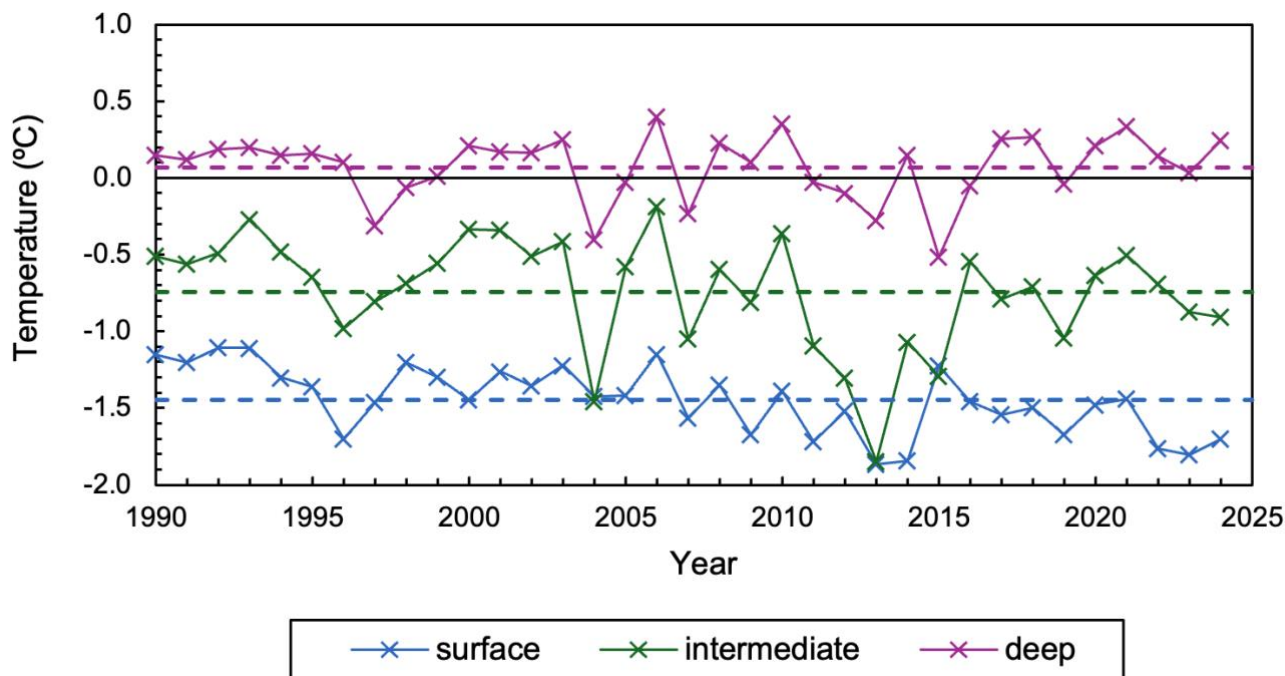
Figure 11: Annual EN4 subsurface ocean temperature across three depth ranges (surface: above 98 m, intermediate: between 110 m and 373 m, deep: below 447 m). Dashed lines show mean temperature at each depth.
