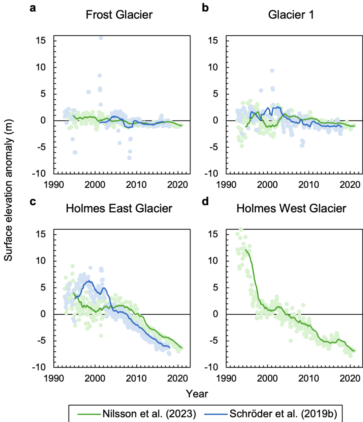
360 Figure 6: Monthly surface elevation anomalies observed in each GL box at (a) Frost Glacier, (b) Glacier 1, (c) Holmes East Glacier, and (d) Holmes West Glacier between 1992 and 2020. Elevation anomalies are calculated relative to the 1992–2017 mean. Bold lines display the 24-month rolling mean.
