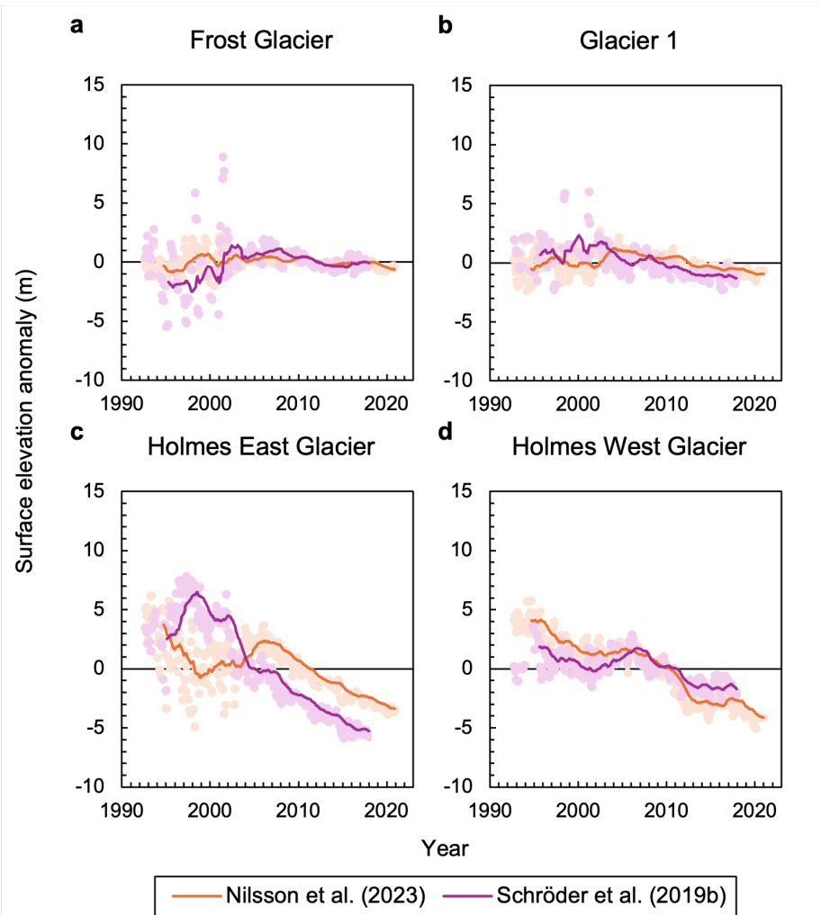
395 Figure 5: Monthly surface elevation anomalies observed in each IN box at (a) Frost Glacier, (b) Glacier 1, (c) Holmes East Glacier, and (d) Holmes West Glacier between 1992 and 2020. Elevation anomalies are calculated relative to the 1992–2017 mean. Bold lines display the 24-month rolling mean.
