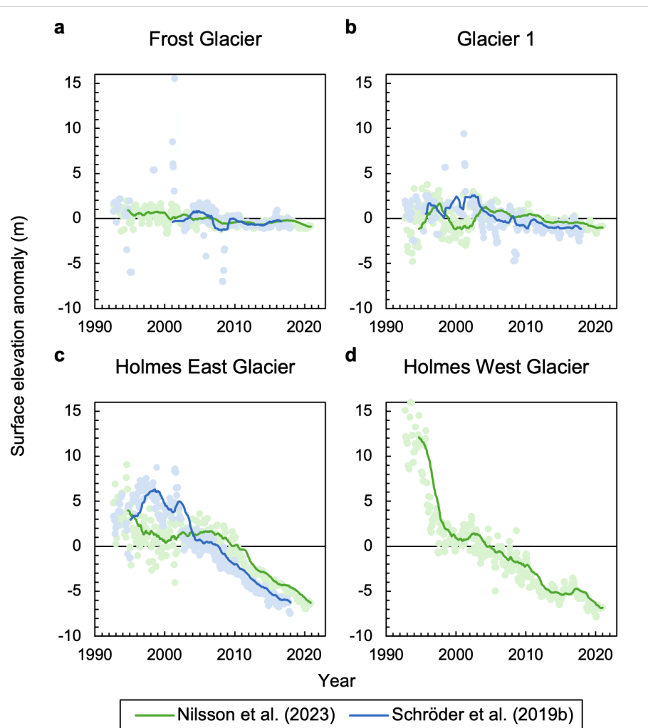
Figure 6: Monthly surface elevation anomalies observed in each GL box at (a) Frost Glacier, (b) Glacier 1, (c) Holmes East Glacier, and (d) Holmes West Glacier between 1992 and 2020. Elevation anomalies are calculated relative to the 1992–2017 mean. Bold lines display the 24-month rolling mean.
