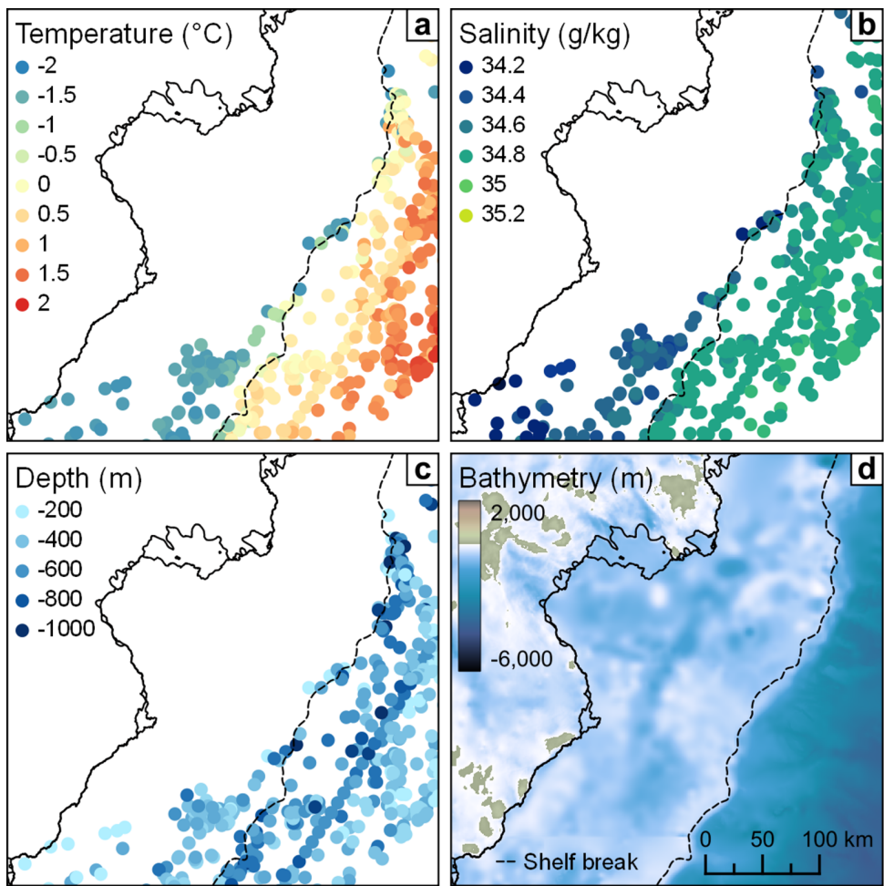
Figure 12: Oceanic properties derived from the MEOP casts and Argo floats between 2004 and 2021 near Porpoise Bay: (a) maximum conservative temperature (°C) observed below 150 m depth at each seal dive, (b) absolute salinity ( \text{g kg}^{-1} ) at the depth of (a), (c) depth of observed maximum temperature (a), (d) bathymetry of the continental shelf from ANTGG (Rignot et al., 2024). Dashed line shows continental shelf break from Amblas (2018) at approximately 600–800 m, solid line shows 2007–2009 ice sheet and shelf edges from MEaSUREs (Mouginot et al., 2017).
