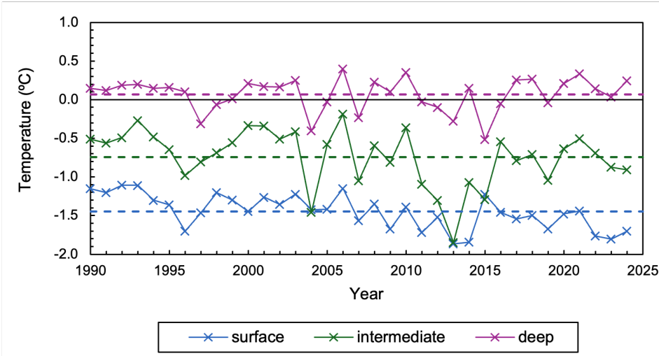
Figure 11: Annual EN4 subsurface ocean temperature across three depth ranges (surface: above 98 m, intermediate: between 110 m and 373 m, deep: below 447 m). Dashed lines show mean temperature at each depth.
