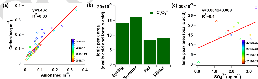
Figure 3. (a) Charge balance between major cations ( \text{Na}^+ + \text{NH}_4^+ + \text{K}^+ + \text{Ca}^{2+} + \text{Mg}^{2+} ) and anions ( \text{Cl}^- + \text{NO}_3^- + \text{SO}_4^{2-} ); (b) seasonal variation of oxalic acid ion peak areas; and (c) correlation between oxalate ion peak area and mass concentration of sulfate in summer. Two scatter plots are fitted with linear regression, the fitting equations and coefficients are shown in the figure.
