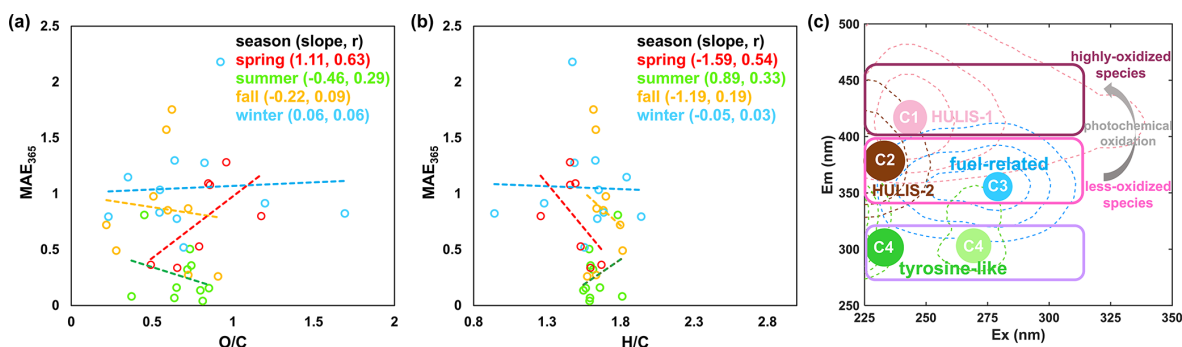
Figure 10. Relationships between optical properties and chemical characteristics. (a, b) Scatterplots of MAE 365 versus O/C and H/C ratios for the four seasons; (c) fluorescence peak positions of chromophores and their potential oxidation state.
