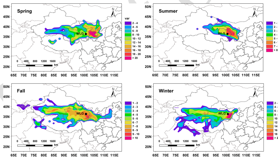
Figure 5. Seasonal concentration-weighted trajectory (CWT) analysis of PM 2.5 mass concentrations and air mass trajectories shown in Fig. 4 performed using MeteInfo software.
