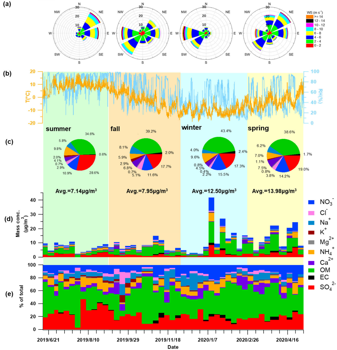
Figure 2. Overview of the dataset used in this study. (a) Wind-rose diagrams for each season; (b) time series of air temperature ( T ) and relative humidity (RH); (c) seasonal average average chemical composition; (d) mass concentration of all measured species, including water-soluble ions (WSIs), organic matter (OM), and elemental carbon (EC); and (e) relative contributions of each species to the total \text{PM}_{2.5} mass.
