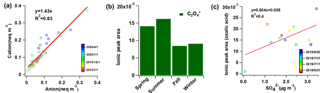
Figure 3. (a) Charge balance between major cations ( \text{Na}^+ + \text{NH}_4^+ + \text{K}^+ + \text{Ca}^{2+} + \text{Mg}^{2+} ) and anions ( \text{Cl}^- + \text{NO}_3^- + \text{SO}_4^{2-} ); (b) seasonal variation of oxalic acid ion peak areas; and (c) correlation between
