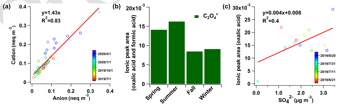
Figure 3. (a) Charge balance between major cations ( \text{Na}^+ + \text{NH}_4^+ + \text{K}^+ + \text{Ca}^{2+} + \text{Mg}^{2+} ) and anions ( \text{Cl}^- + \text{NO}_3^- + \text{SO}_4^{2-} ); (b) seasonal variation of oxalic acid ion peak areas; and (c) correlation between oxalate ion peak area and mass concentration of sulfate in summer. Two scatter plots are fitted with linear regression, the fitting equations and coefficients are shown in the figure.
