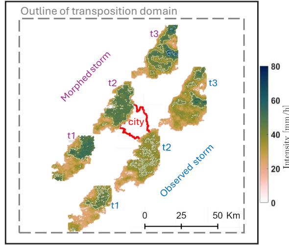
Figure 3. SST transposition domain (grey dashed box) around an interested city area (red polygon). Observed storm trajectory for a single historical storm (blue), sampled here at three-hourly intervals for clarity, and DSQM-based projected future trajectory of the same storm (purple) after randomized transposition via SST. The transposed future storm exhibits higher mean areal rainfall intensity and spatial heterogeneity.
