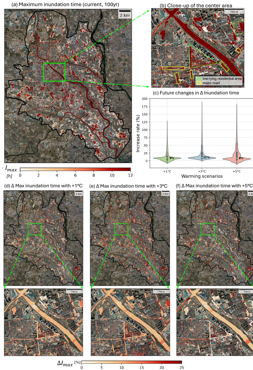
Figure 8. (a) The inundation duration for 100-yr rainfall return level under the current climate, (b) zoom-in part in the BMC centre, (c) future changes of inundation duration under different regional warming levels, and its spatial distribution of those changes within BMC region under 1°C (d), 3°C (e), 5°C (f) warming levels. Basemaps are derived from ESRI World Imagery (Credit: Esri, TomTom, Garmin, FAO, NOAA, USGS, © OpenStreetMap contributors, and the GIS User Community).
