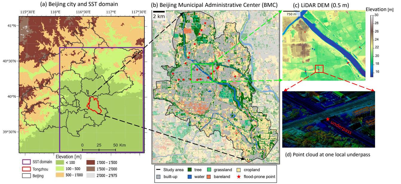
Figure 4. (a) Location map, showing Beijing Municipality area (black polygons), Beijing Municipal Administrative Center (BMC, red polygon), and the SST transposition domain (purple box). (b) Land use and historical flood-prone points within BMC. (c) Zoom in to a 0.5 m digital elevation model (DEM) in the BMC center. (d) Zoom in on a LiDAR point cloud data at a local underpass used for DEM generation.
