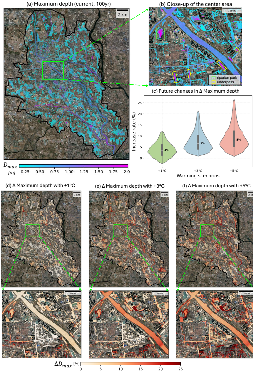
Figure 7. (a) The maximum flood depth for 100-yr rainfall return level under the current climate, (b) zoom-in part in the BMC centre, (c) future changes of maximum flood depth under different regional warming levels, and its spatial distribution of those changes within BMC region under 1°C (d), 3°C (e), 5°C (f) warming levels. Basemaps are derived from ESRI World Imagery (Credit: Esri, TomTom, Garmin, FAO, NOAA, USGS, © OpenStreetMap contributors, and the GIS User Community).
