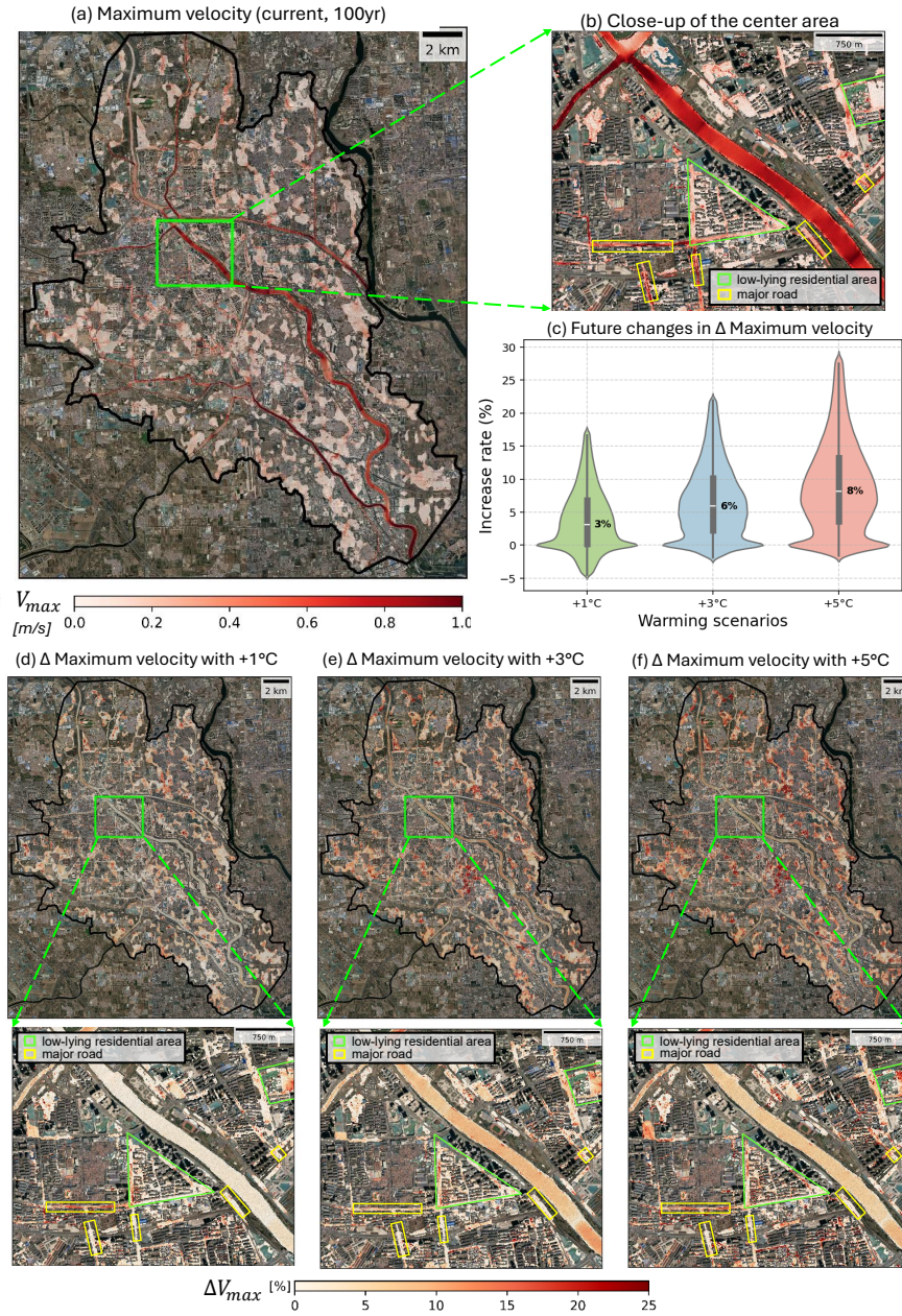
Figure 9. (a) The maximum velocity for 100-yr rainfall return level under the current climate, (b) zoom-in to the BMC center, (c) future changes of maximum velocity under different regional future warming levels, and its spatial distribution of those changes within BMC region under 1°C (d), 3°C (e), 5°C (f) warming level. Basemaps are derived from ESRI World Imagery (Credit: Esri, TomTom, Garmin, FAO, NOAA, USGS, © OpenStreetMap contributors, and the GIS User Community).
