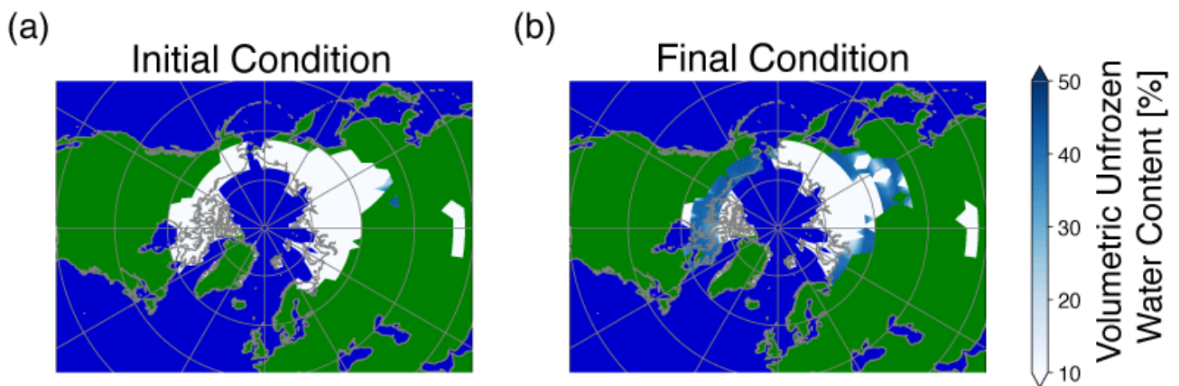
380 Figure 5: Soil property in the bottom layer (4–14m) in (a) the piControl experiment and (b) the last year of the NEC6 experiment. Note that GSAT is nearly the same between the two states. Regions in white indicate ice areas, while in blue indicate sherbet areas where the water phase change is undergoing (darker blue denotes a larger amount of unfrozen water).
