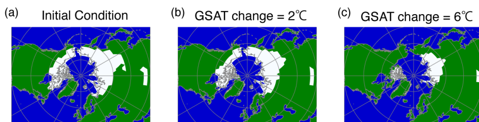
Figure 2: Permafrost areas (white) at different stages in the flat10 experiment: (a) initial state, (b) warmed state when the GSAT increases by 2°C, and (c) warmed state when the GSAT increases by is 6°C.
