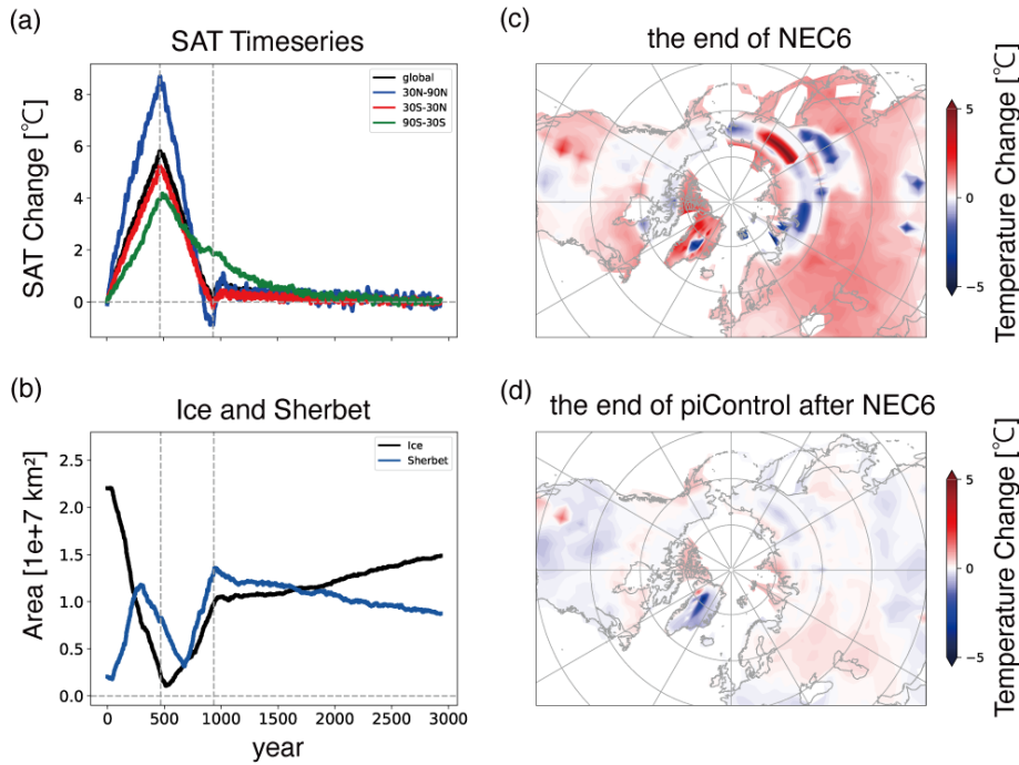
Figure 11 (a)(b) Timeseries in flat10, NEC6, and the 2000-year piControl run after NEC6 experiment.
