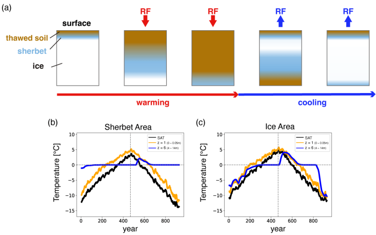
Figure 7: Schematic explaining hysteresis and irreversibility of the physical permafrost during thawing and re-freezing. (a) Five rectangular panels show the vertical cross sections of the soil, representing the initial state of warming (leftmost), followed by the warming states during and at the end of the flat10 experiment, and the two cooling states during and at the end of the NEC experiment. Radiative forcing and the SAT changes are shown by arrows. (b), (c) Timeseries of annual-mean temperature in regions where the bottom layer (4–14m) is sherbet (b: 68° N, 87° W) and ice (c: 71° N, 171° E) at the end of the NEC6 experiment. The black curves represent the SAT, and the brown and blue curves represent the ground temperature at the surface layer (0–0.05m) and the bottom layer, respectively. The vertical dashed line indicates the year when the flat10 run is switched to NEC6.
