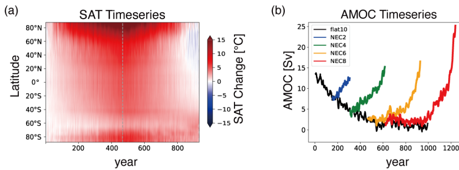
635 Figure 10: Hysteresis and irreversibility in the large-scale climate indicator. (a) Response of annual- and zonal-mean surface air temperature in flat10 and NEC6. The vertical dashed line indicates the year when flat10 is switched to NEC6. (b) Timeseries of the 11-year running mean AMOC index (maximum value of the meridional stream function at 34° N) in flat10 and the four NEC experiments. The color convention 640 follows Fig. 1.
