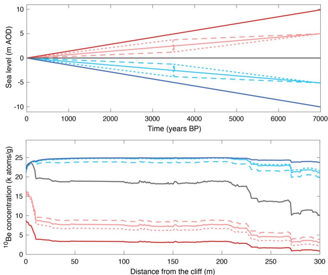
Figure 7. Impact of relative sea level on a non-eroding rocky shore. Top panel shows seven simplified sea-level histories over the last 7000 years: stable (grey), rising linearly (by 5 m solid light blue, and by 10 m solid dark blue), rising with upward/downward step change (dashed/dotted light blue), falling linearly (by 5 m solid light red, and by 10 m solid dark red), and falling with downward/upward step change (dashed/dotted light red). Bottom panel shows the corresponding nuclide concentrations across the platform. No surface cover, down-wearing or cliff retreat is applied for these scenarios. The overall magnitude and across-platform distribution of nuclide concentrations differs between stable, linearly rising and linearly falling scenarios. Adding a step change to the trend has an impact, albeit relatively small. Differences between scenarios of rising sea level are smaller than between those of falling sea level as the platform is influenced less by water shielding over time.
