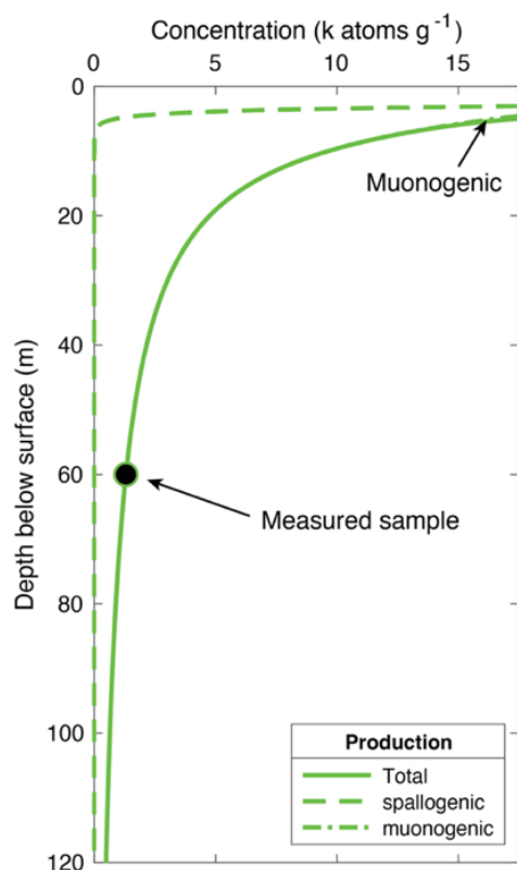
Figure 1. Application of the ‘cosmogenic inheritance’ model. The model’s predicted nuclide concentration is in green, shown with depth for different production pathways (lines) and for total production at the sample depth (circle). The measured inheritance sample has a ^{10}\text{Be} concentration of 1304 \pm 268 atoms \text{g}^{-1} (mean and standard deviation), which was collected 60 m below the surface of the cliff top. The model perfectly fits the measured concentration (chi-squared = 0) from a best-fit steady-state surface erosion rate of <0.001 (non-zero) \text{mm yr}^{-1} .
