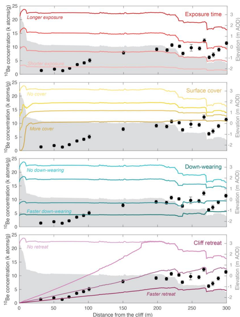
Figure 2. Impact of different parameters on nuclide concentrations across a real-world platform. The top panel shows shorter to longer exposure time (which corresponds to total model time): 1, 3, 5 and 7 ka. For the rest of the panels, exposure time is 7 ka and only the featured parameter is included and changed. The second panel shows no beach cover and increasing cover depth (density = 1.6 \text{ g cm}^{-3} ): 0, 0.5, 1 and 5 m. The third panel shows no down-wearing to increasing down-wearing rates: 0, 0.05, 0.22 (present-day observed rate at the site) and 0.5 \text{ mm yr}^{-1} . The bottom panel shows no cliff retreat to increasing retreat rates: 0, 0.027 (present-day observed rate), 0.05 and 0.5 \text{ m yr}^{-1} . The black symbols are measured concentrations from the site in North Yorkshire UK, and the background shading shows the elevation profile of the platform (Swirad et al., 2020). The same relative sea-level history is used for all scenarios.
