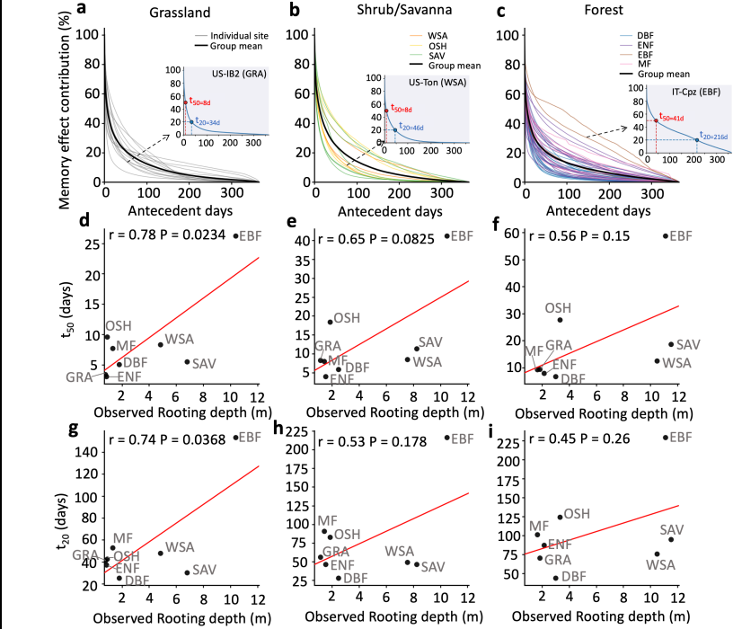
Figure 8. Memory effect decay of antecedent contributions across plant functional groups and its relationship with observed rooting depth. Panels a–c show the decay of normalized antecedent memory contributions with increasing lag days for grassland, shrub/savanna, and forest groups, respectively. Thin colored or gray lines denote individual sites, and thick black lines denote the group mean. Insets illustrate representative examples of decay timescales, with t_{50} and t_{20} defined as the antecedent days required for the normalized memory contribution to decay to 50% and 20% of its initial value (100%), respectively. Panels d–f show the relationships between observed rooting depth and t_{50} aggregated at the 20th, 50th, and 80th percentiles, respectively, while panels g–i show the corresponding relationships for t_{20} . Red lines indicate linear fits across plant functional types, with Pearson's r and corresponding P values shown in each panel. Following the rooting-depth comparison approach of Stocker et al. (2023), observed rooting depth and memory decay timescales were aggregated at the
